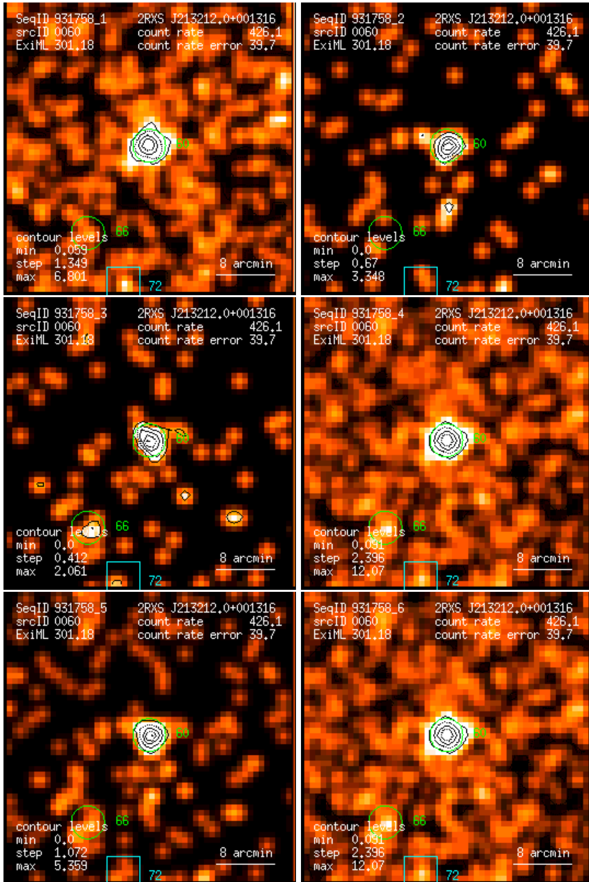
Figure 60: RASS 931758: detection 0060: band rate images, Gaussian filter: (1) PSPC channels 11 – 41, (2) 52 – 90, (3) 91 – 201, (4) 11 – 235, (5) 52 – 201, (6) 11 – 201. Broad band rates in counts/ks. Band rate contour levels in counts/ks/arcmin 2 .
