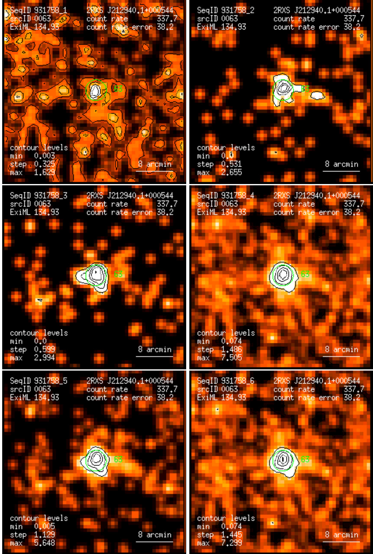
Figure 63: RASS 931758: detection 0063: band rate images, Gaussian filter: (1) PSPC channels 11 – 41, (2) 52 – 90, (3) 91 – 201, (4) 11 – 235, (5) 52 – 201, (6) 11 – 201. Broad band rates in counts/ks. Band rate contour levels in counts/ks/arcmin 2 .
