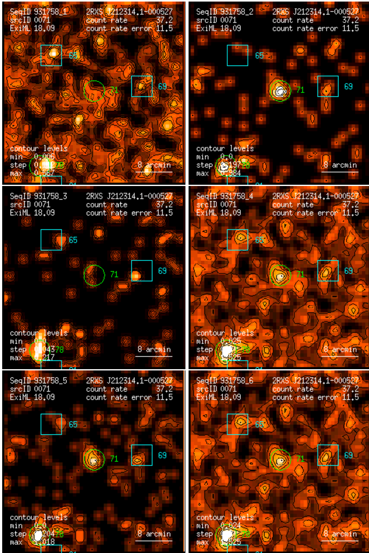
Figure 71: RASS 931758: detection 0071: band rate images, Gaussian filter: (1) PSPC channels 11 – 41, (2) 52 – 90, (3) 91 – 201, (4) 11 – 235, (5) 52 – 201, (6) 11 – 201. Broad band rates in counts/ks. Band rate contour levels in counts/ks/arcmin 2 .
