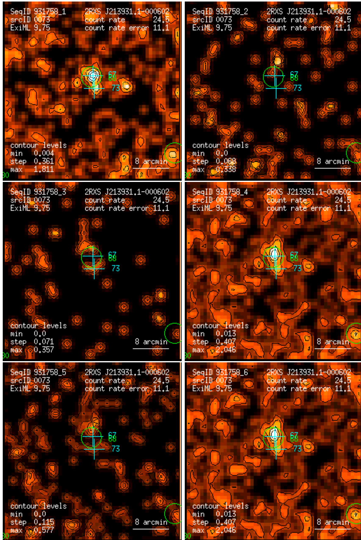
Figure 73: RASS 931758: detection 0073: band rate images, Gaussian filter: (1) PSPC channels 11 – 41, (2) 52 – 90, (3) 91 – 201, (4) 11 – 235, (5) 52 – 201, (6) 11 – 201. Broad band rates in counts/ks. Band rate contour levels in counts/ks/arcmin 2 .
