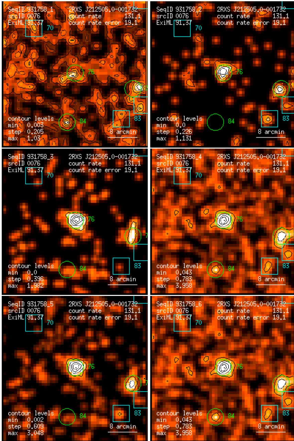
Figure 76: RASS 931758: detection 0076: band rate images, Gaussian filter: (1) PSPC channels 11 – 41, (2) 52 – 90, (3) 91 – 201, (4) 11 – 235, (5) 52 – 201, (6) 11 – 201. Broad band rates in counts/ks. Band rate contour levels in counts/ks/arcmin 2 .
