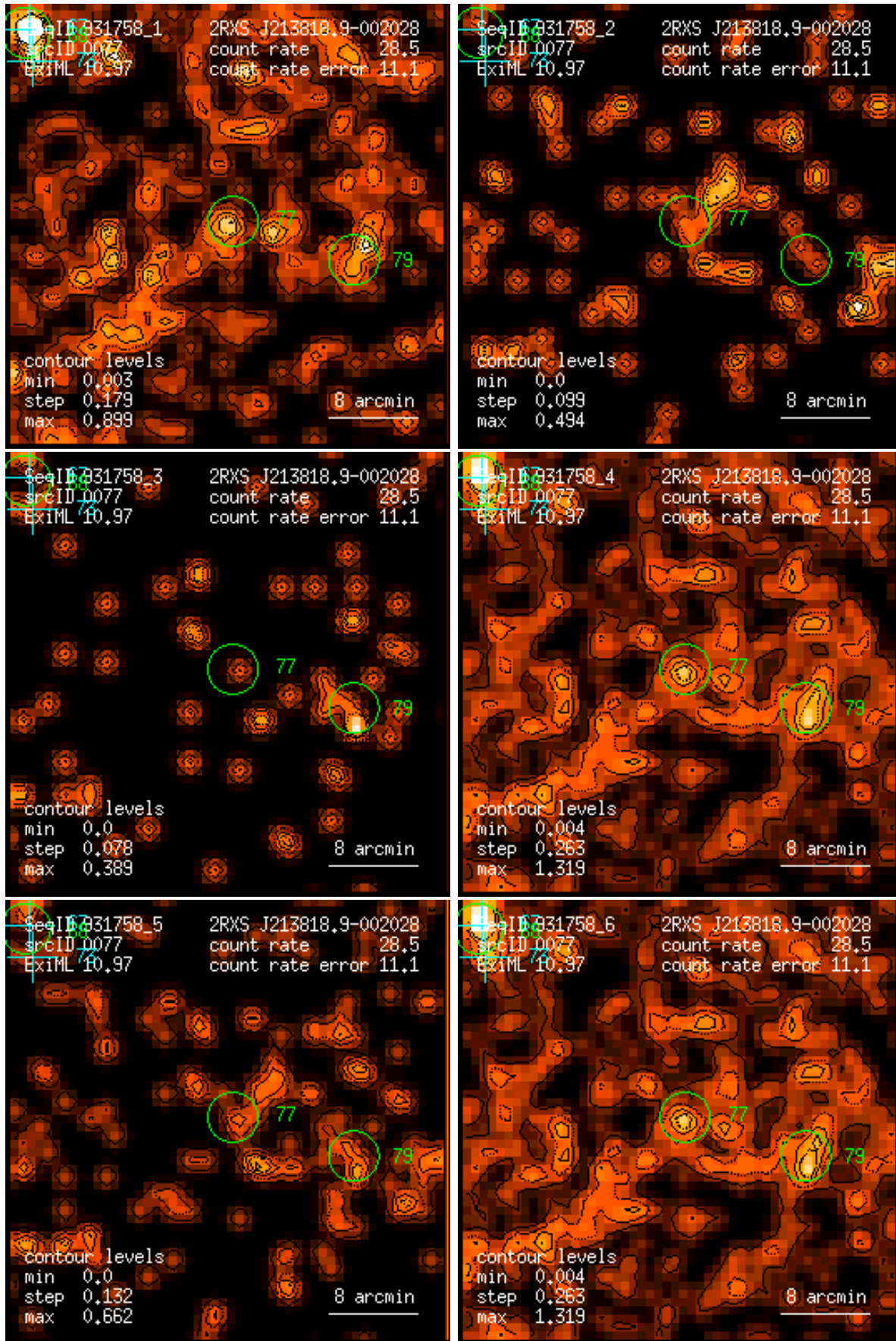
Figure 77: RASS 931758: detection 0077: band rate images, Gaussian filter: (1) PSPC channels 11 – 41, (2) 52 – 90, (3) 91 – 201, (4) 11 – 235, (5) 52 – 201, (6) 11 – 201. Broad band rates in counts/ks. Band rate contour levels in counts/ks/arcmin 2 .
