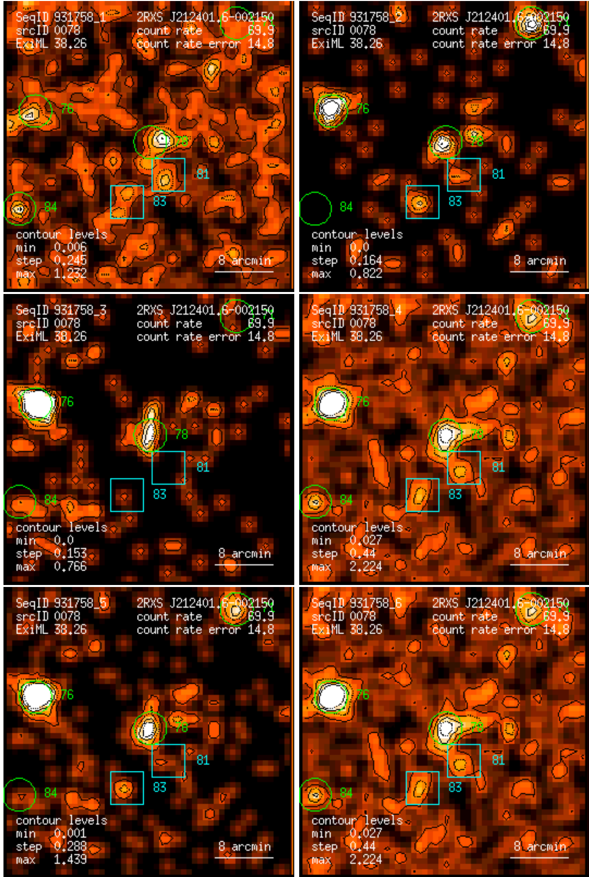
Figure 78: RASS 931758: detection 0078: band rate images, Gaussian filter: (1) PSPC channels 11 – 41, (2) 52 – 90, (3) 91 – 201, (4) 11 – 235, (5) 52 – 201, (6) 11 – 201. Broad band rates in counts/ks. Band rate contour levels in counts/ks/arcmin 2 .
