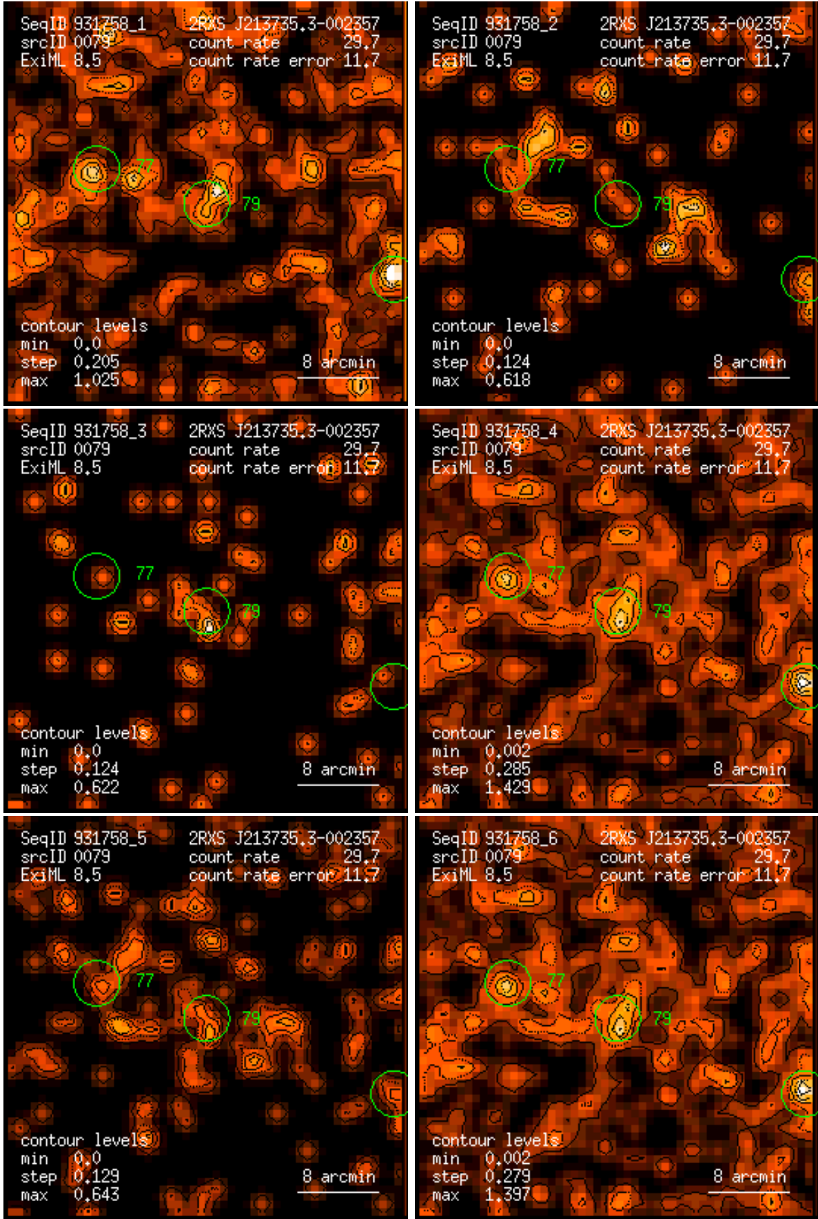
Figure 79: RASS 931758: detection 0079: band rate images, Gaussian filter: (1) PSPC channels 11 – 41, (2) 52 – 90, (3) 91 – 201, (4) 11 – 235, (5) 52 – 201, (6) 11 – 201. Broad band rates in counts/ks. Band rate contour levels in counts/ks/arcmin 2 .
