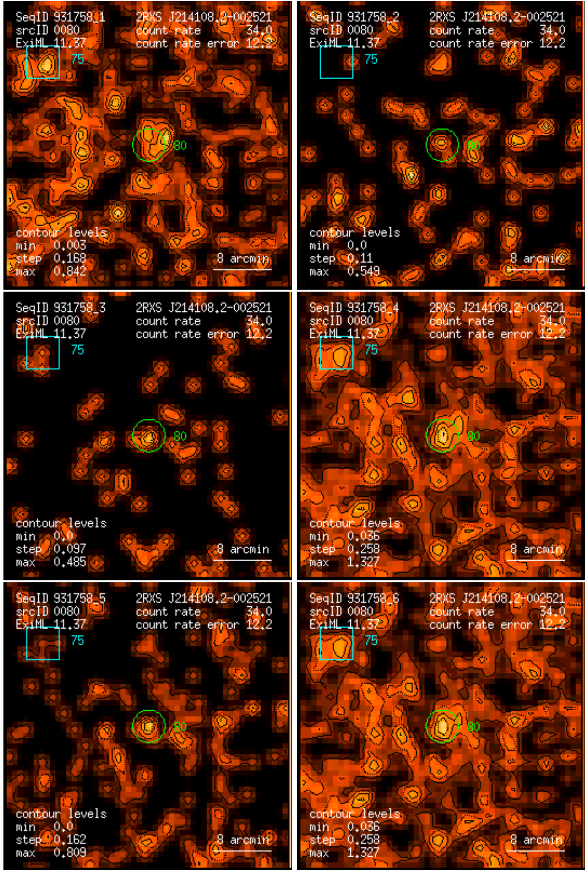
Figure 80: RASS 931758: detection 0080: band rate images, Gaussian filter: (1) PSPC channels 11 – 41, (2) 52 – 90, (3) 91 – 201, (4) 11 – 235, (5) 52 – 201, (6) 11 – 201. Broad band rates in counts/ks. Band rate contour levels in counts/ks/arcmin 2 .
