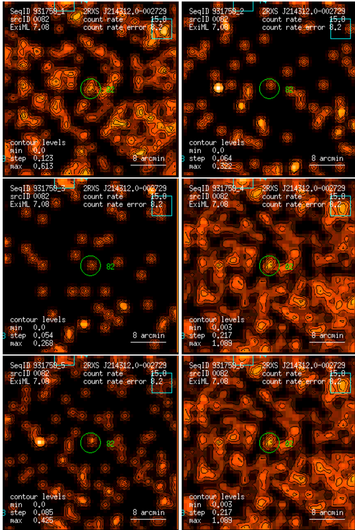
Figure 82: RASS 931758: detection 0082: band rate images, Gaussian filter: (1) PSPC channels 11 – 41, (2) 52 – 90, (3) 91 – 201, (4) 11 – 235, (5) 52 – 201, (6) 11 – 201. Broad band rates in counts/ks. Band rate contour levels in counts/ks/arcmin 2 .
