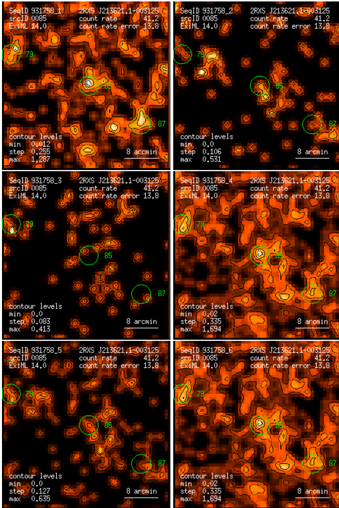
Figure 85: RASS 931758: detection 0085: band rate images, Gaussian filter: (1) PSPC channels 11 – 41, (2) 52 – 90, (3) 91 – 201, (4) 11 – 235, (5) 52 – 201, (6) 11 – 201. Broad band rates in counts/ks. Band rate contour levels in counts/ks/arcmin 2 .
