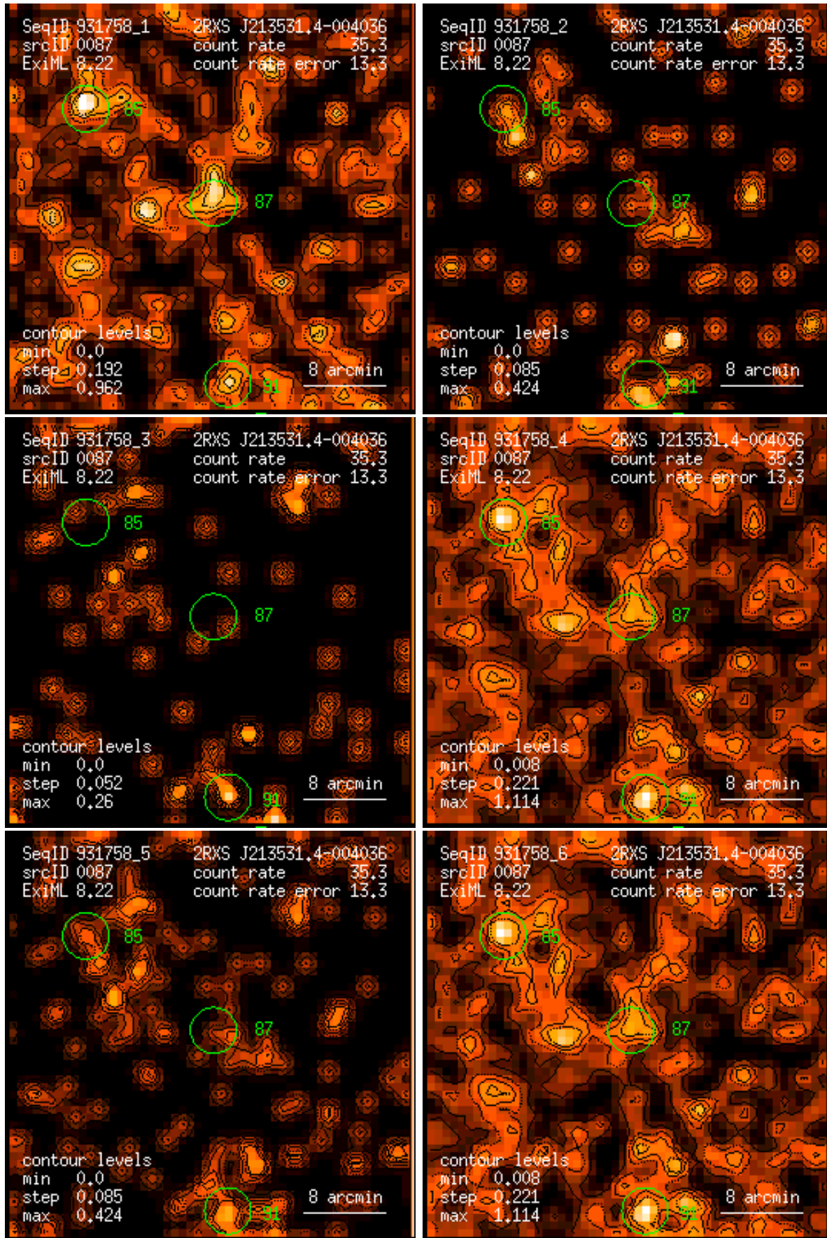
Figure 87: RASS 931758: detection 0087: band rate images, Gaussian filter: (1) PSPC channels 11 – 41, (2) 52 – 90, (3) 91 – 201, (4) 11 – 235, (5) 52 – 201, (6) 11 – 201. Broad band rates in counts/ks. Band rate contour levels in counts/ks/arcmin 2 .
