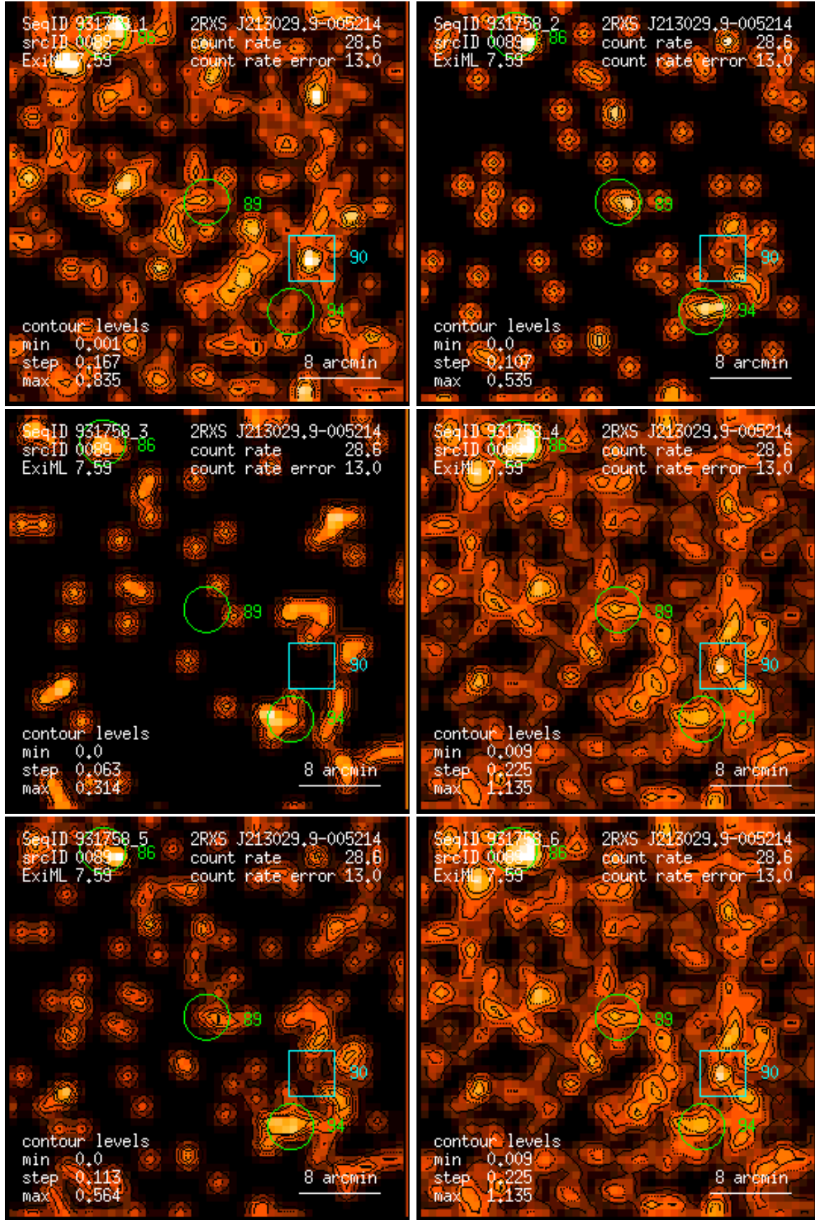
Figure 89: RASS 931758: detection 0089: band rate images, Gaussian filter: (1) PSPC channels 11 – 41, (2) 52 – 90, (3) 91 – 201, (4) 11 – 235, (5) 52 – 201, (6) 11 – 201. Broad band rates in counts/ks. Band rate contour levels in counts/ks/arcmin 2 .
