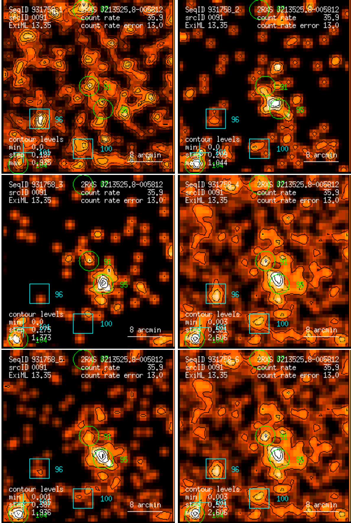
Figure 91: RASS 931758: detection 0091: band rate images, Gaussian filter: (1) PSPC channels 11 – 41, (2) 52 – 90, (3) 91 – 201, (4) 11 – 235, (5) 52 – 201, (6) 11 – 201. Broad band rates in counts/ks. Band rate contour levels in counts/ks/arcmin 2 .
