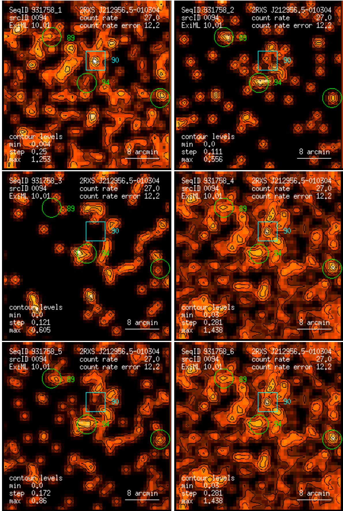
Figure 94: RASS 931758: detection 0094: band rate images, Gaussian filter: (1) PSPC channels 11 – 41, (2) 52 – 90, (3) 91 – 201, (4) 11 – 235, (5) 52 – 201, (6) 11 – 201. Broad band rates in counts/ks. Band rate contour levels in counts/ks/arcmin 2 .
