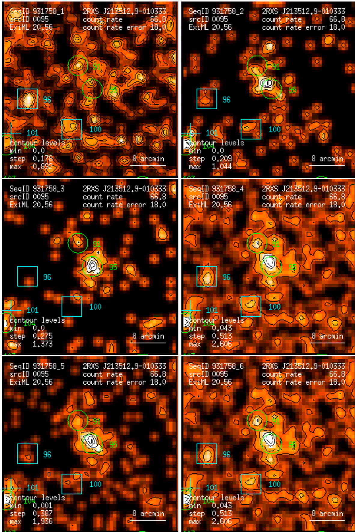
Figure 95: RASS 931758: detection 0095: band rate images, Gaussian filter: (1) PSPC channels 11 – 41, (2) 52 – 90, (3) 91 – 201, (4) 11 – 235, (5) 52 – 201, (6) 11 – 201. Broad band rates in counts/ks. Band rate contour levels in counts/ks/arcmin 2 .
