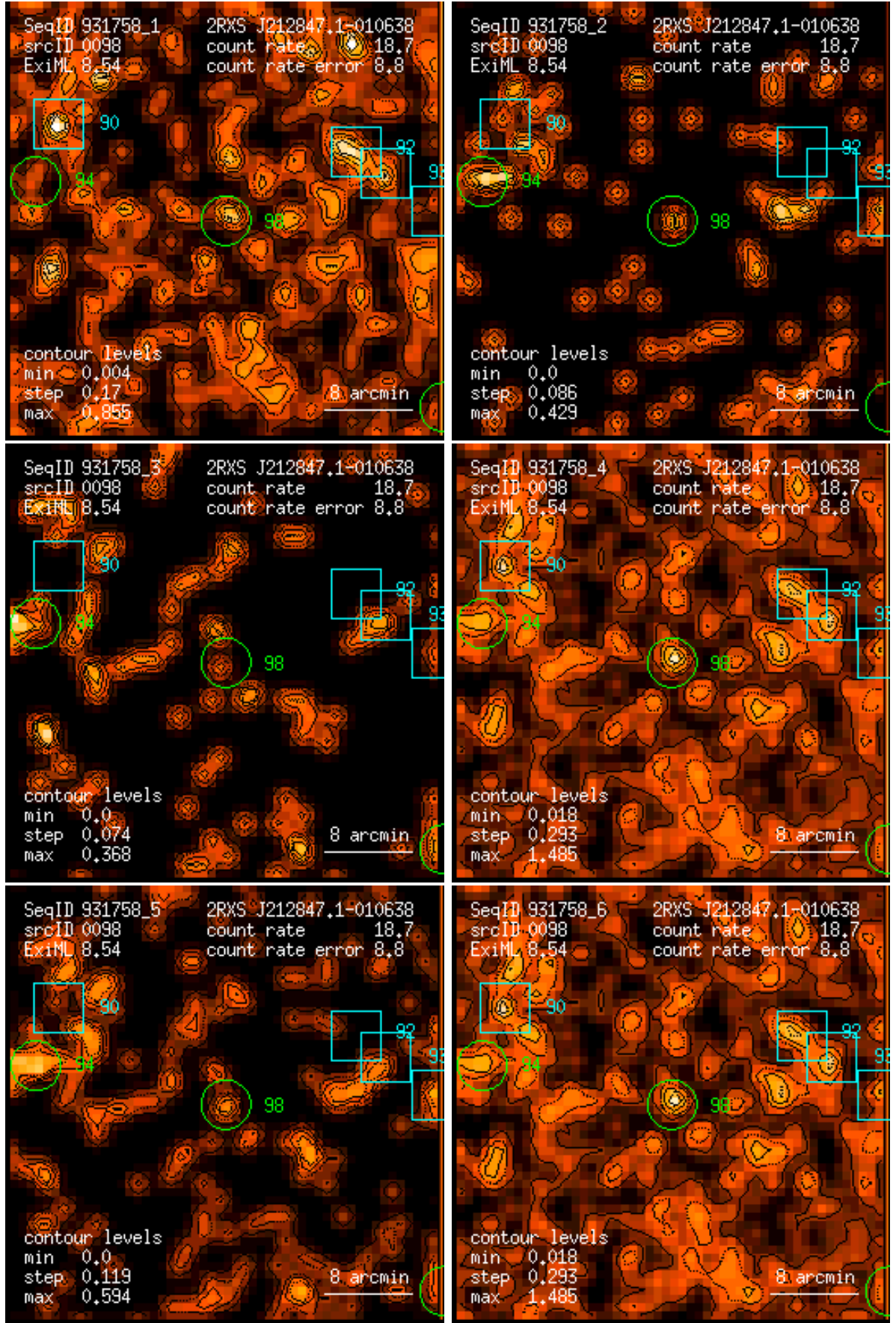
Figure 98: RASS 931758: detection 0098: band rate images, Gaussian filter: (1) PSPC channels 11 – 41, (2) 52 – 90, (3) 91 – 201, (4) 11 – 235, (5) 52 – 201, (6) 11 – 201. Broad band rates in counts/ks. Band rate contour levels in counts/ks/arcmin 2 .
