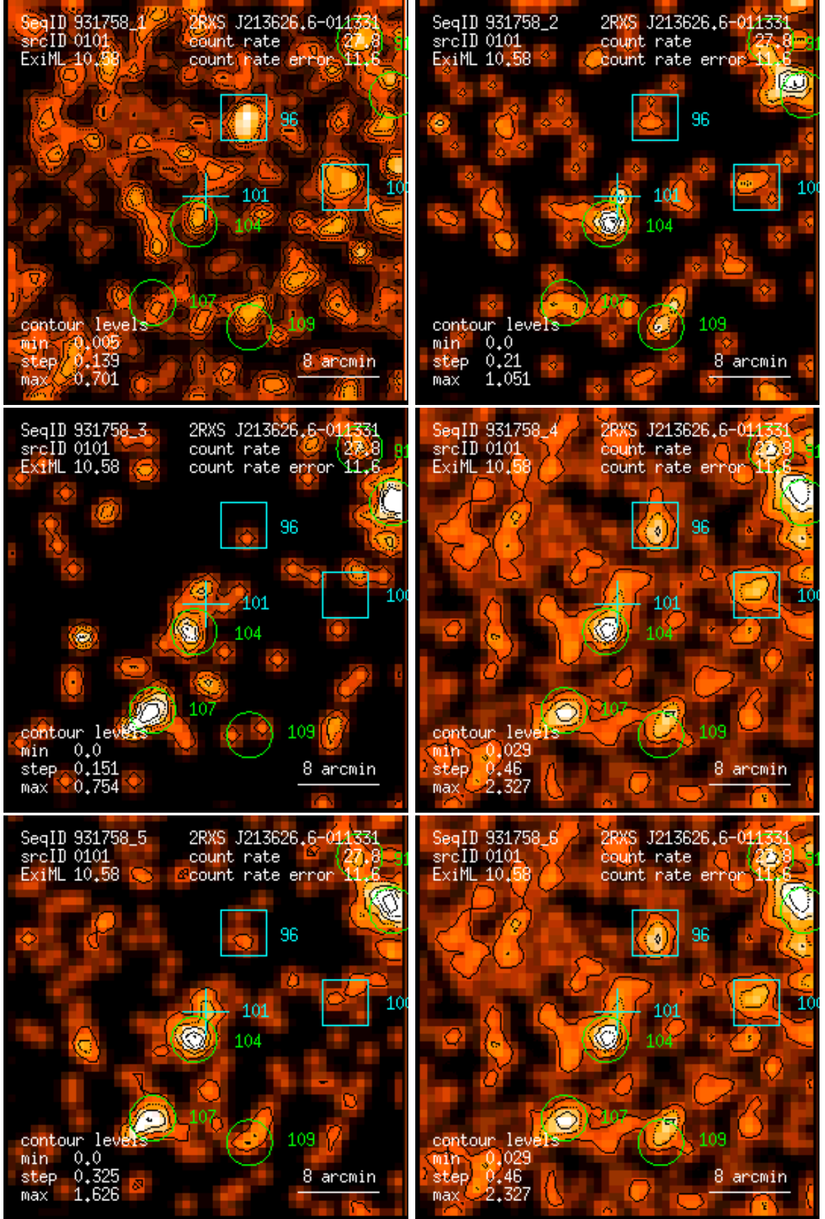
Figure 101: RASS 931758: detection 0101: band rate images, Gaussian filter: (1) PSPC channels 11 – 41, (2) 52 – 90, (3) 91 – 201, (4) 11 – 235, (5) 52 – 201, (6) 11 – 201. Broad band rates in counts/ks. Band rate contour levels in counts/ks/arcmin 2 .
