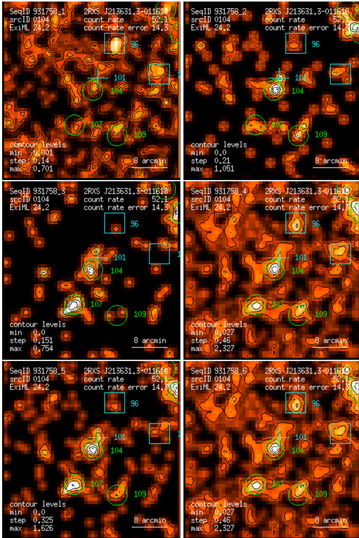
Figure 104: RASS 931758: detection 0104: band rate images, Gaussian filter: (1) PSPC channels 11 – 41, (2) 52 – 90, (3) 91 – 201, (4) 11 – 235, (5) 52 – 201, (6) 11 – 201. Broad band rates in counts/ks. Band rate contour levels in counts/ks/arcmin 2 .
