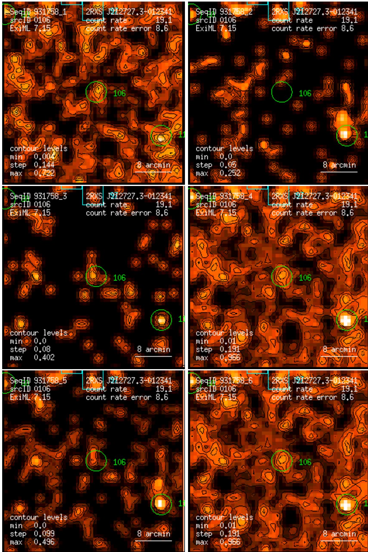
Figure 106: RASS 931758: detection 0106: band rate images, Gaussian filter: (1) PSPC channels 11 – 41, (2) 52 – 90, (3) 91 – 201, (4) 11 – 235, (5) 52 – 201, (6) 11 – 201. Broad band rates in counts/ks. Band rate contour levels in counts/ks/arcmin 2 .
