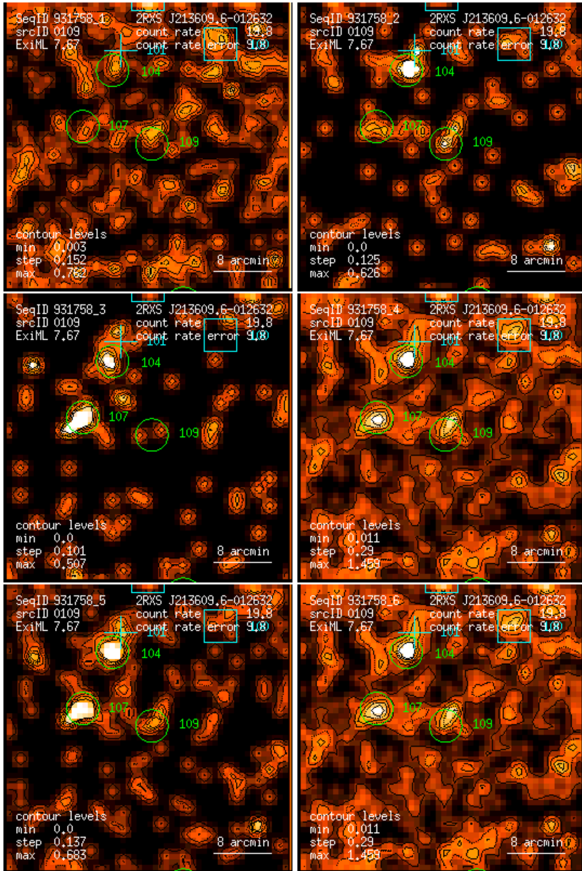
Figure 109: RASS 931758: detection 0109: band rate images, Gaussian filter: (1) PSPC channels 11 – 41, (2) 52 – 90, (3) 91 – 201, (4) 11 – 235, (5) 52 – 201, (6) 11 – 201. Broad band rates in counts/ks. Band rate contour levels in counts/ks/arcmin 2 .
