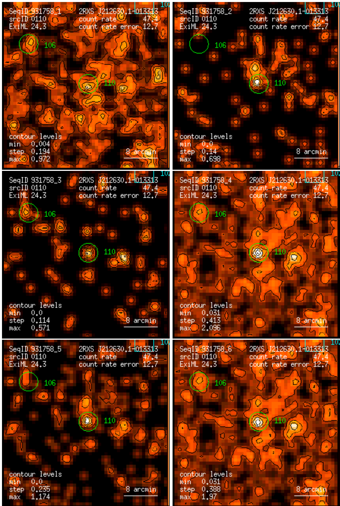
Figure 110: RASS 931758: detection 0110: band rate images, Gaussian filter: (1) PSPC channels 11 – 41, (2) 52 – 90, (3) 91 – 201, (4) 11 – 235, (5) 52 – 201, (6) 11 – 201. Broad band rates in counts/ks. Band rate contour levels in counts/ks/arcmin 2 .
