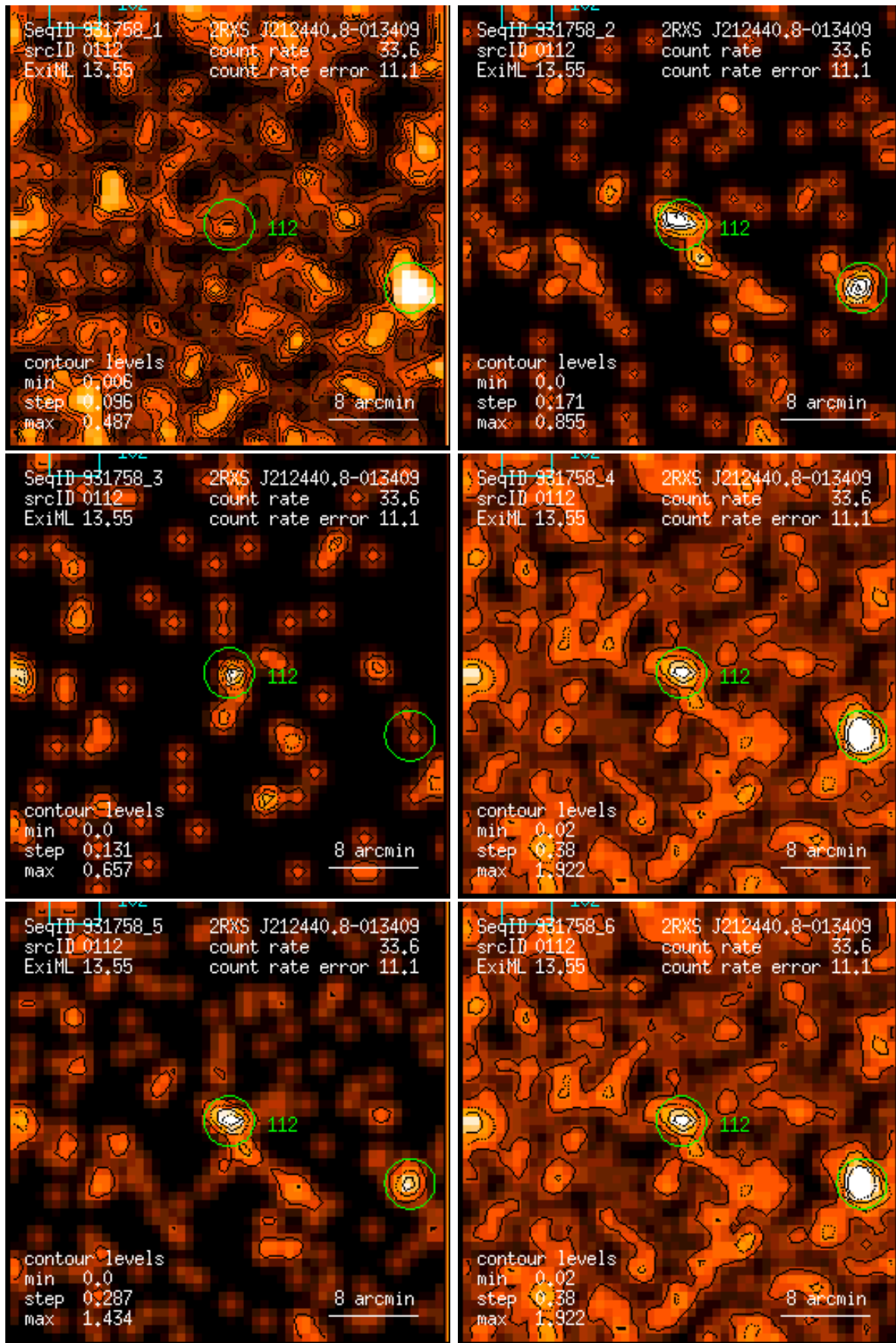
Figure 112: RASS 931758: detection 0112: band rate images, Gaussian filter: (1) PSPC channels 11 – 41, (2) 52 – 90, (3) 91 – 201, (4) 11 – 235, (5) 52 – 201, (6) 11 – 201. Broad band rates in counts/ks. Band rate contour levels in counts/ks/arcmin 2 .
