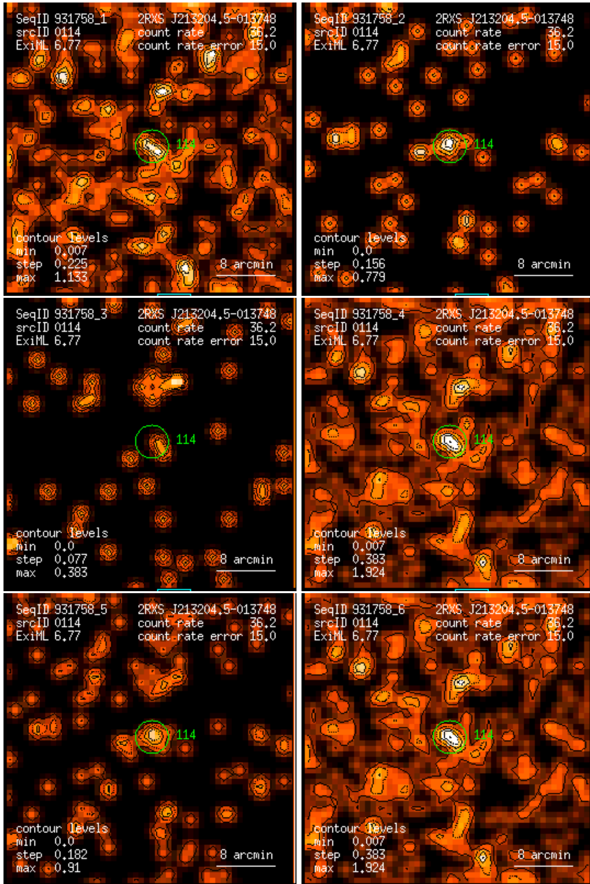
Figure 114: RASS 931758: detection 0114: band rate images, Gaussian filter: (1) PSPC channels 11 – 41, (2) 52 – 90, (3) 91 – 201, (4) 11 – 235, (5) 52 – 201, (6) 11 – 201. Broad band rates in counts/ks. Band rate contour levels in counts/ks/arcmin 2 .
