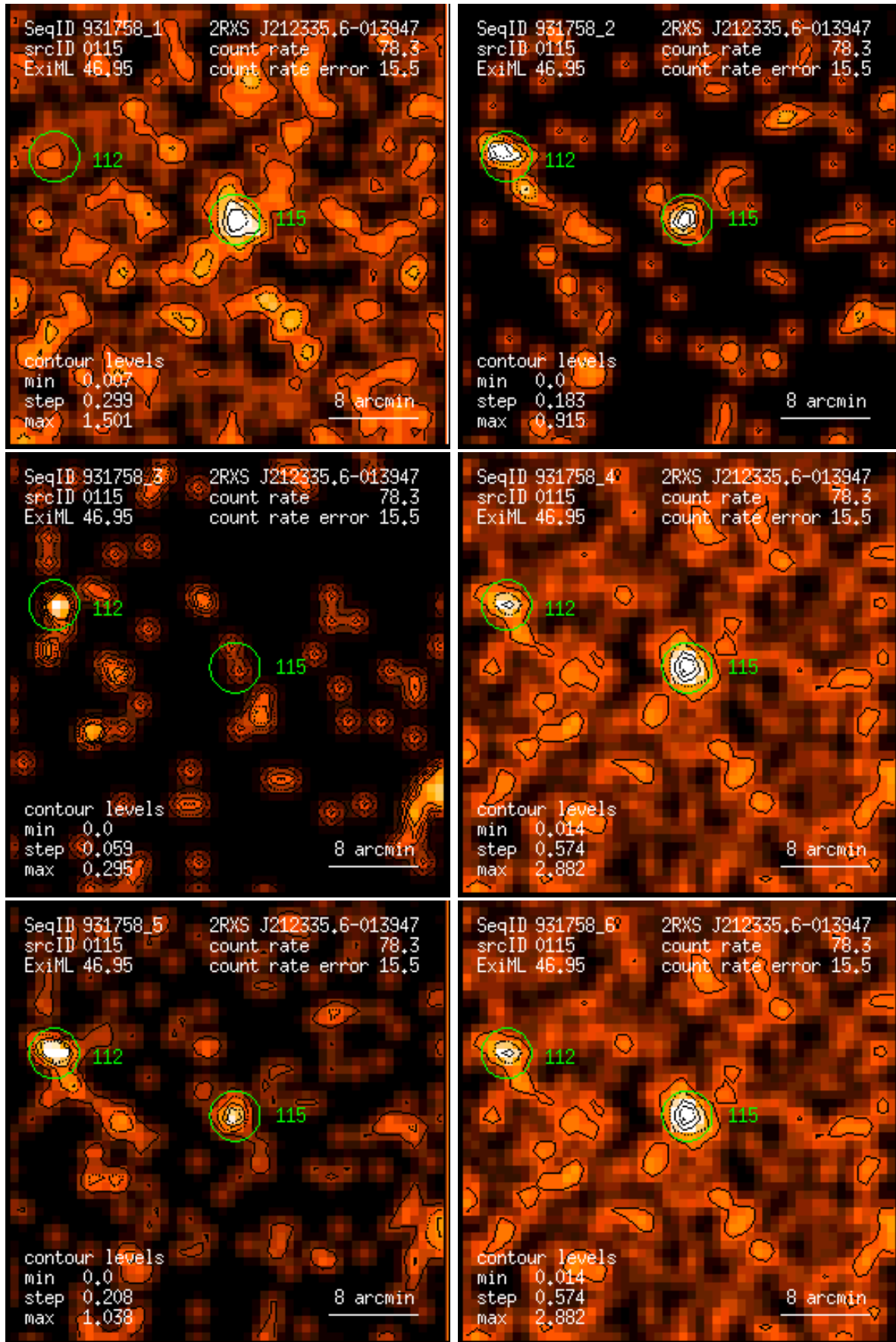
Figure 115: RASS 931758: detection 0115: band rate images, Gaussian filter: (1) PSPC channels 11 – 41, (2) 52 – 90, (3) 91 – 201, (4) 11 – 235, (5) 52 – 201, (6) 11 – 201. Broad band rates in counts/ks. Band rate contour levels in counts/ks/arcmin 2 .
