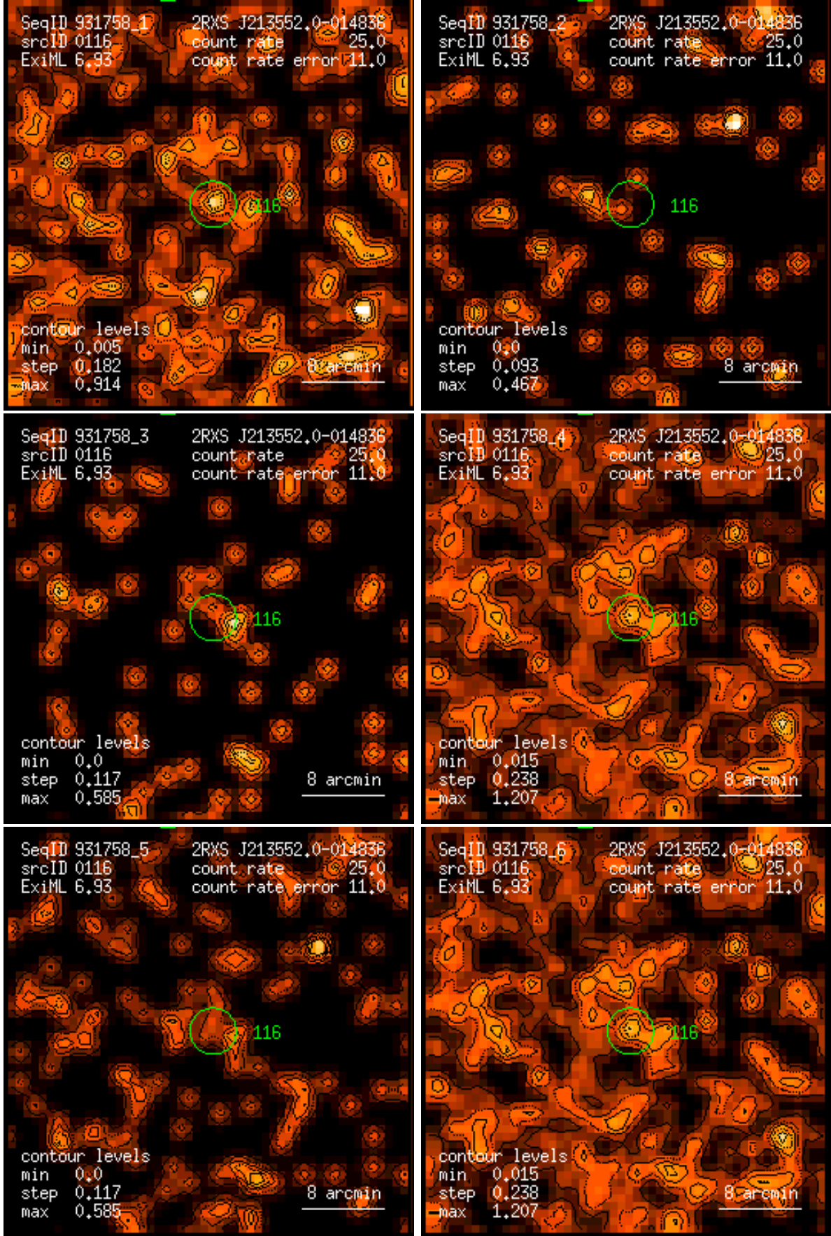
Figure 116: RASS 931758: detection 0116: band rate images, Gaussian filter: (1) PSPC channels 11 – 41, (2) 52 – 90, (3) 91 – 201, (4) 11 – 235, (5) 52 – 201, (6) 11 – 201. Broad band rates in counts/ks. Band rate contour levels in counts/ks/arcmin 2 .
