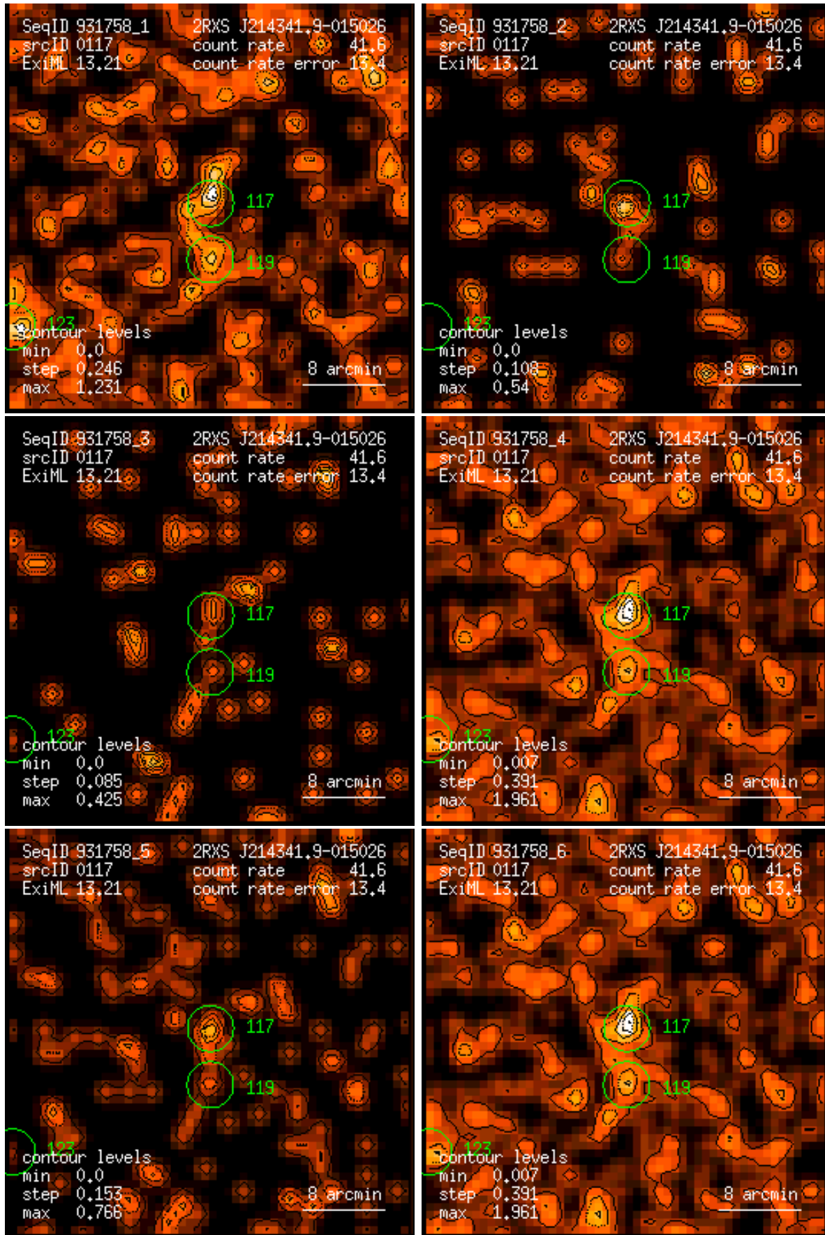
Figure 117: RASS 931758: detection 0117: band rate images, Gaussian filter: (1) PSPC channels 11 – 41, (2) 52 – 90, (3) 91 – 201, (4) 11 – 235, (5) 52 – 201, (6) 11 – 201. Broad band rates in counts/ks. Band rate contour levels in counts/ks/arcmin 2 .
