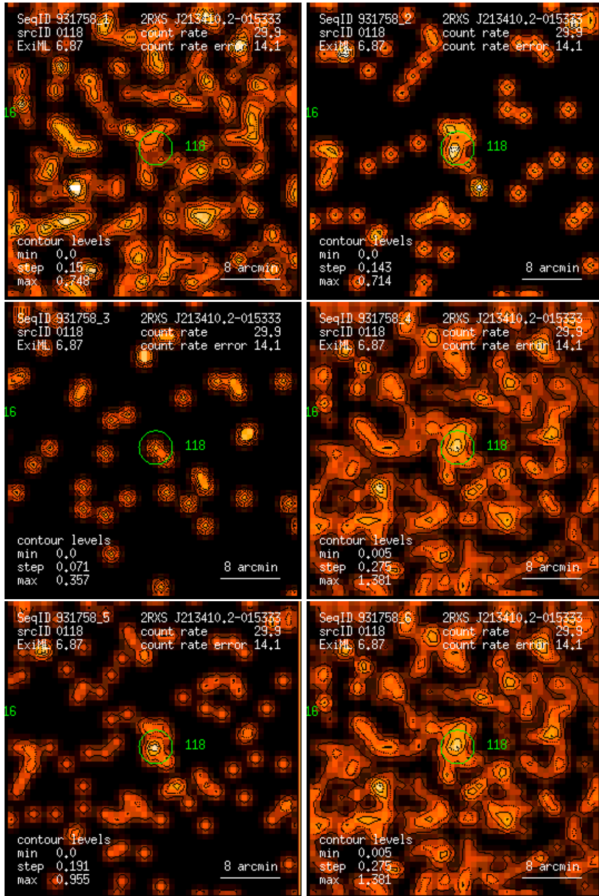
Figure 118: RASS 931758: detection 0118: band rate images, Gaussian filter: (1) PSPC channels 11 – 41, (2) 52 – 90, (3) 91 – 201, (4) 11 – 235, (5) 52 – 201, (6) 11 – 201. Broad band rates in counts/ks. Band rate contour levels in counts/ks/arcmin 2 .
