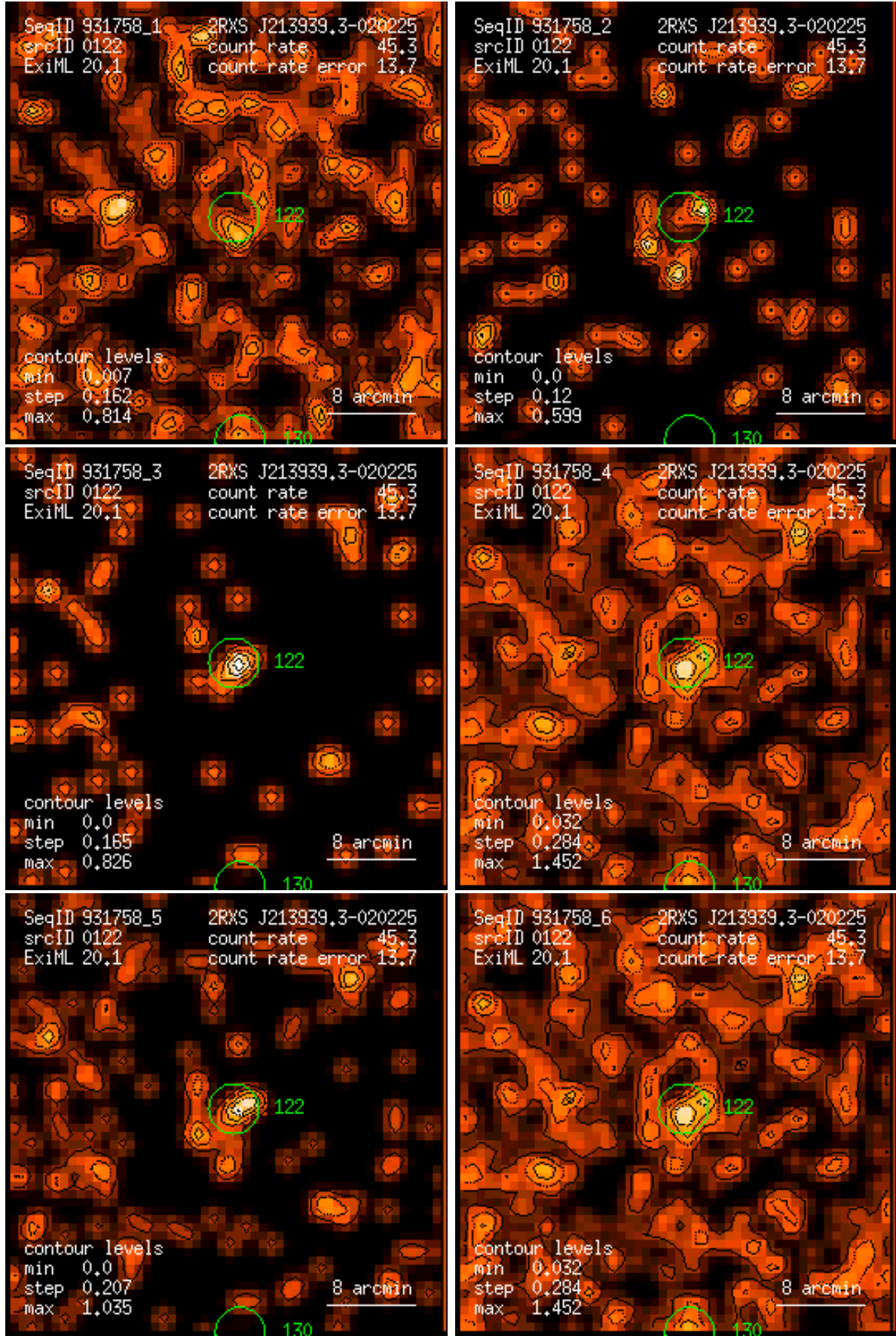
Figure 122: RASS 931758: detection 0122: band rate images, Gaussian filter: (1) PSPC channels 11 – 41, (2) 52 – 90, (3) 91 – 201, (4) 11 – 235, (5) 52 – 201, (6) 11 – 201. Broad band rates in counts/ks. Band rate contour levels in counts/ks/arcmin 2 .
