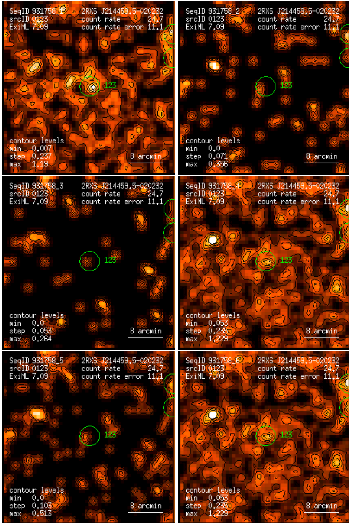
Figure 123: RASS 931758: detection 0123: band rate images, Gaussian filter: (1) PSPC channels 11 – 41, (2) 52 – 90, (3) 91 – 201, (4) 11 – 235, (5) 52 – 201, (6) 11 – 201. Broad band rates in counts/ks. Band rate contour levels in counts/ks/arcmin 2 .
