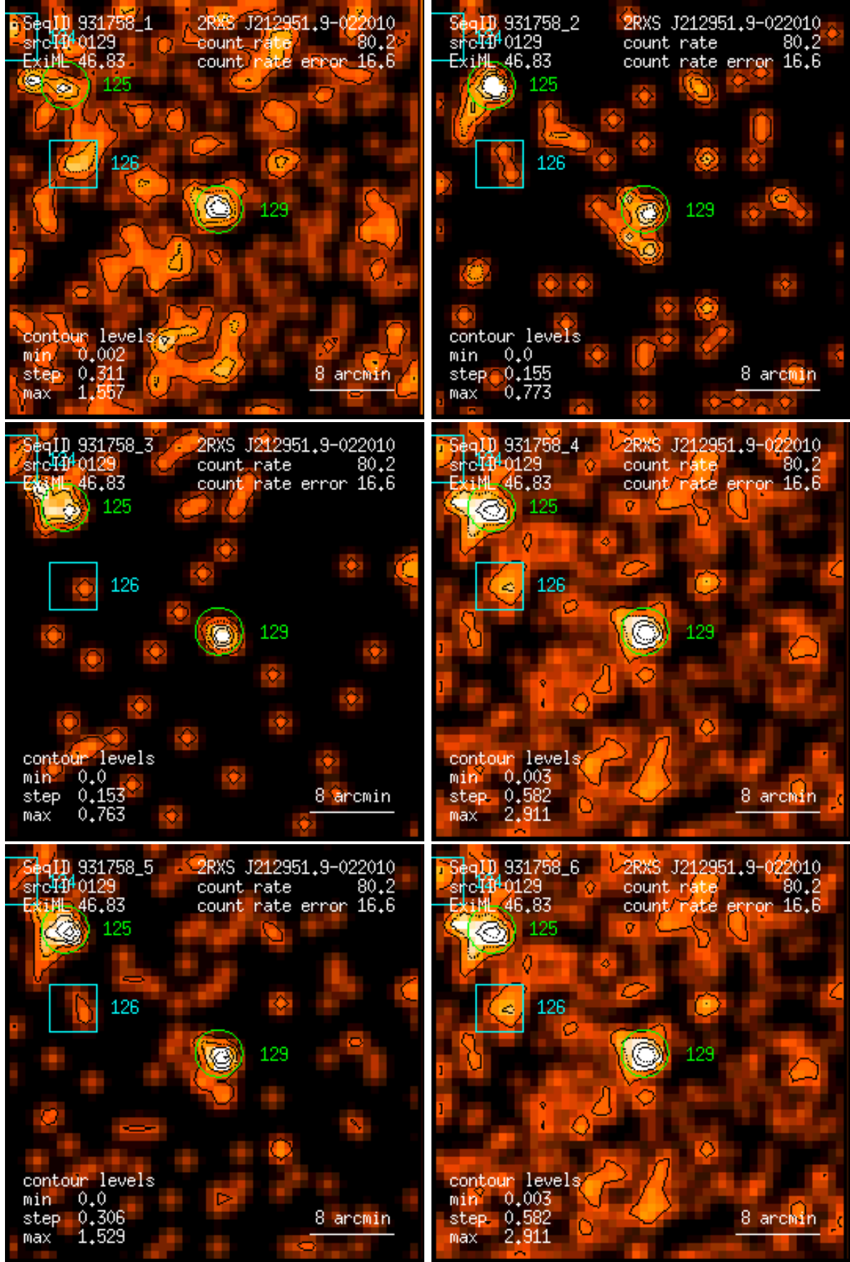
Figure 129: RASS 931758: detection 0129: band rate images, Gaussian filter: (1) PSPC channels 11 – 41, (2) 52 – 90, (3) 91 – 201, (4) 11 – 235, (5) 52 – 201, (6) 11 – 201. Broad band rates in counts/ks. Band rate contour levels in counts/ks/arcmin 2 .
