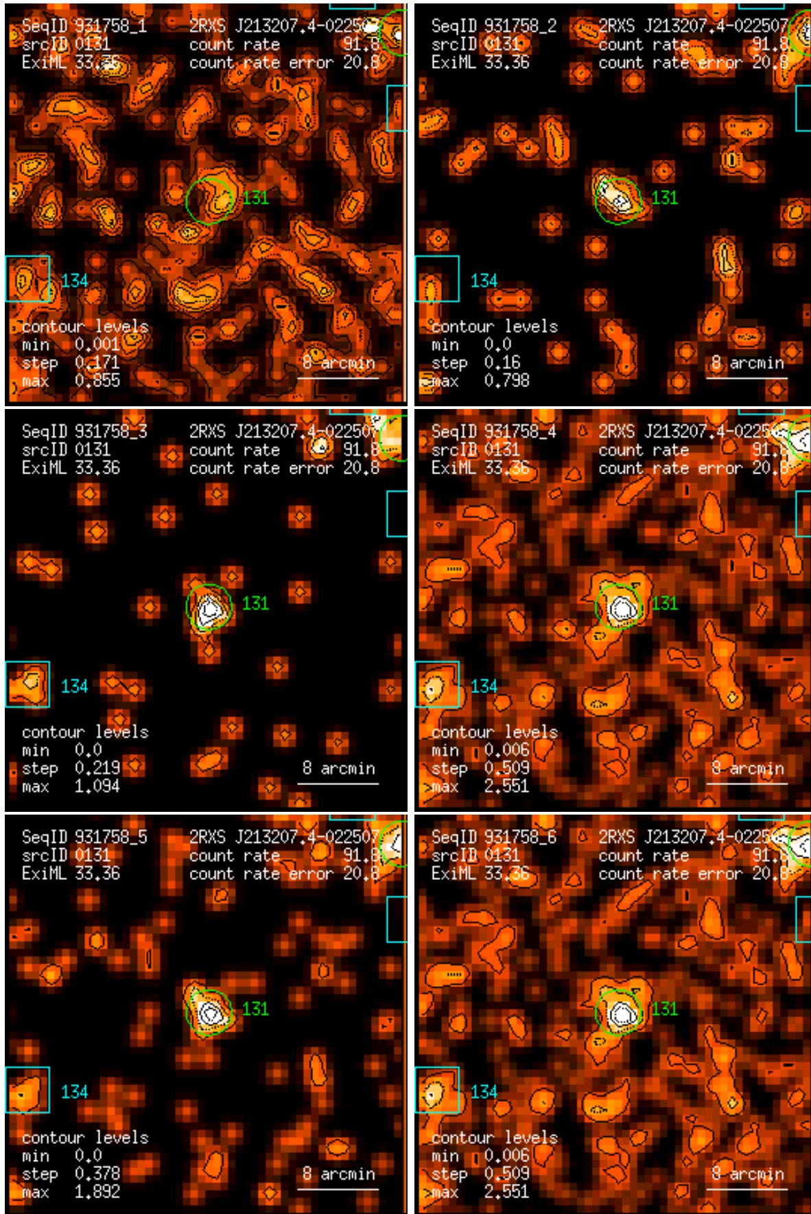
Figure 131: RASS 931758: detection 0131: band rate images, Gaussian filter: (1) PSPC channels 11 – 41, (2) 52 – 90, (3) 91 – 201, (4) 11 – 235, (5) 52 – 201, (6) 11 – 201. Broad band rates in counts/ks. Band rate contour levels in counts/ks/arcmin 2 .
