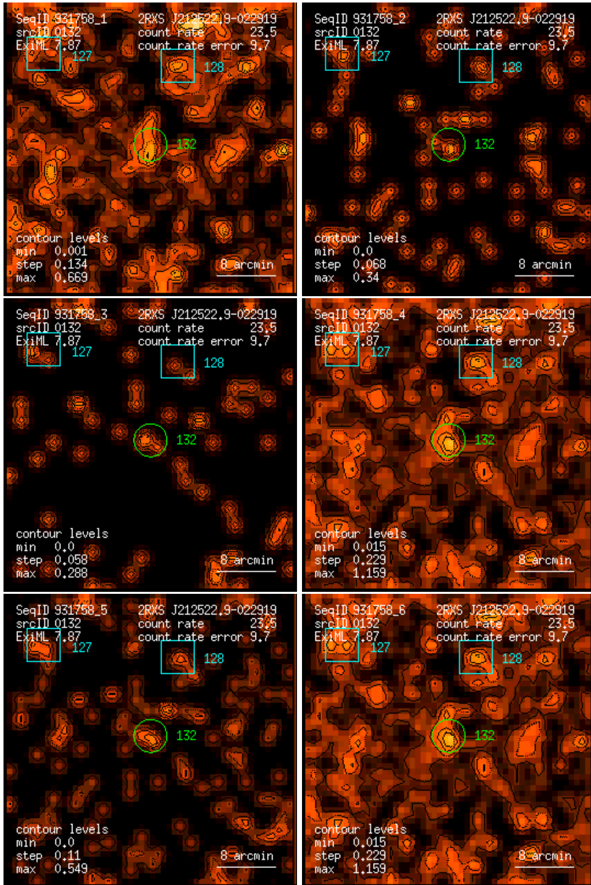
Figure 132: RASS 931758: detection 0132: band rate images, Gaussian filter: (1) PSPC channels 11 – 41, (2) 52 – 90, (3) 91 – 201, (4) 11 – 235, (5) 52 – 201, (6) 11 – 201. Broad band rates in counts/ks. Band rate contour levels in counts/ks/arcmin 2 .
