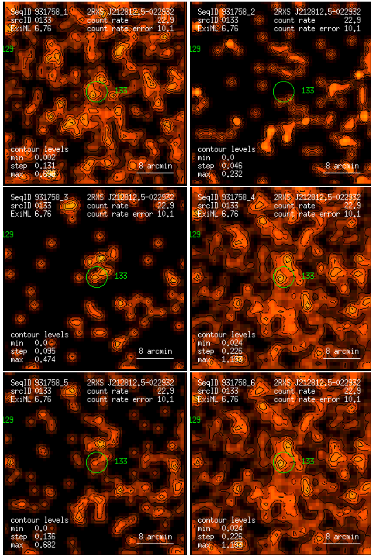
Figure 133: RASS 931758: detection 0133: band rate images, Gaussian filter: (1) PSPC channels 11 – 41, (2) 52 – 90, (3) 91 – 201, (4) 11 – 235, (5) 52 – 201, (6) 11 – 201. Broad band rates in counts/ks. Band rate contour levels in counts/ks/arcmin 2 .
