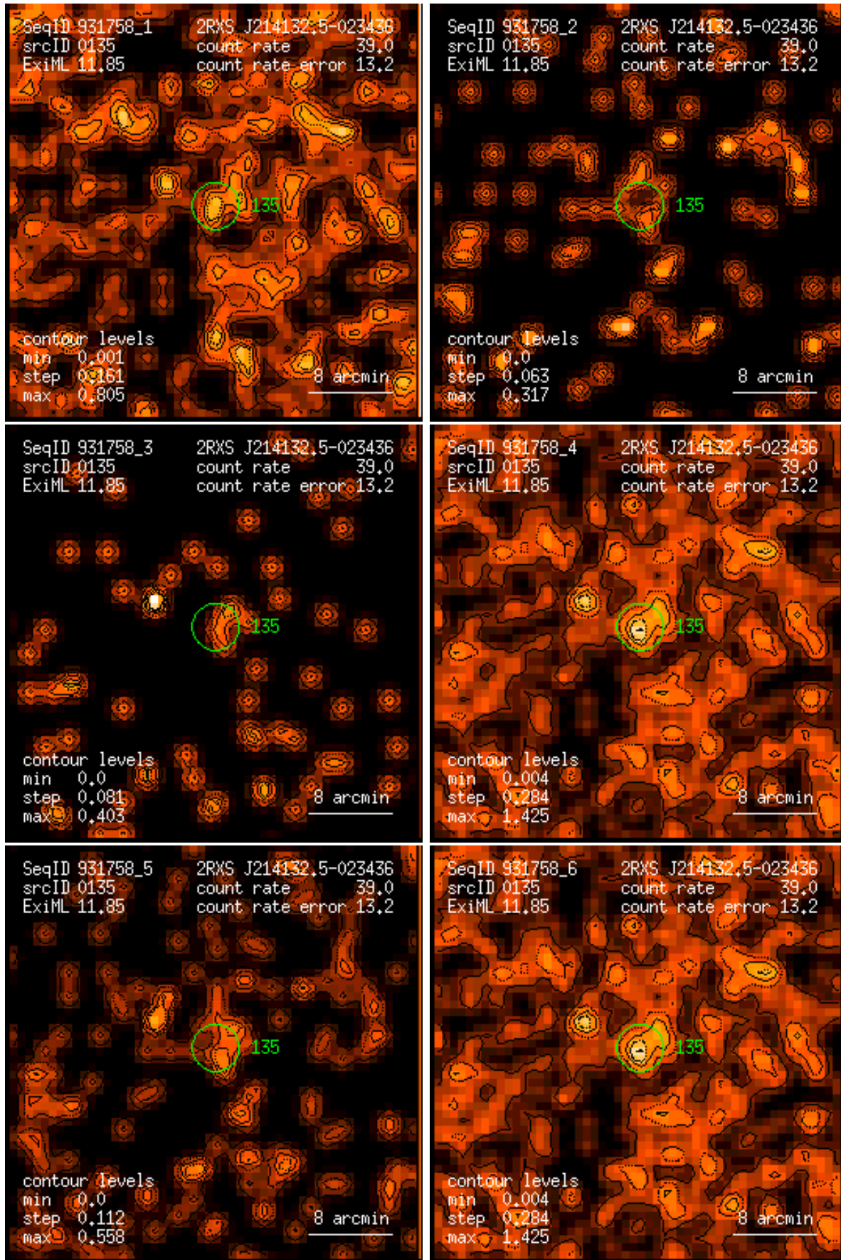
Figure 135: RASS 931758: detection 0135: band rate images, Gaussian filter: (1) PSPC channels 11 – 41, (2) 52 – 90, (3) 91 – 201, (4) 11 – 235, (5) 52 – 201, (6) 11 – 201. Broad band rates in counts/ks. Band rate contour levels in counts/ks/arcmin 2 .
