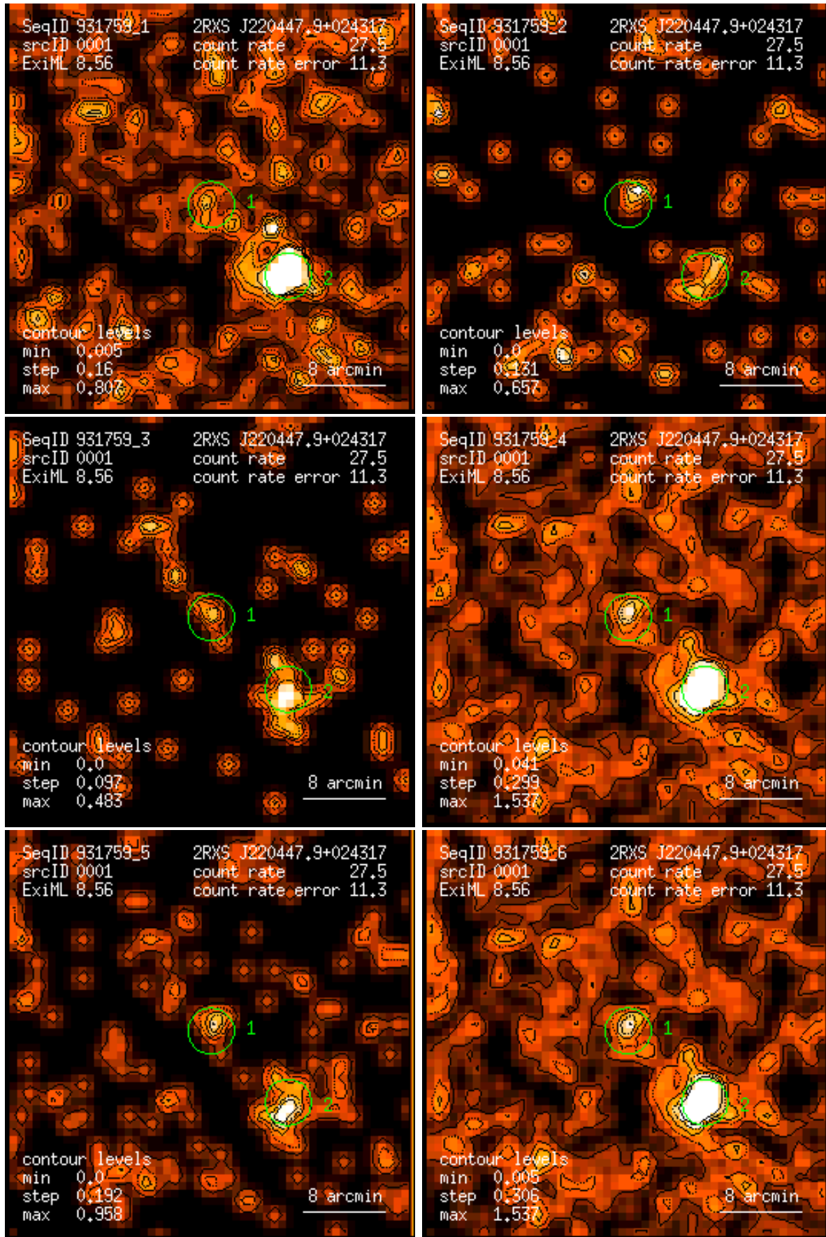
Figure 1: RASS 931759: detection 0001: band rate images, Gaussian filter: (1) PSPC channels 11 – 41, (2) 52 – 90, (3) 91 – 201, (4) 11 – 235, (5) 52 – 201, (6) 11 – 201. Broad band rates in counts/ks. Band rate contour levels in counts/ks/arcmin 2 .
