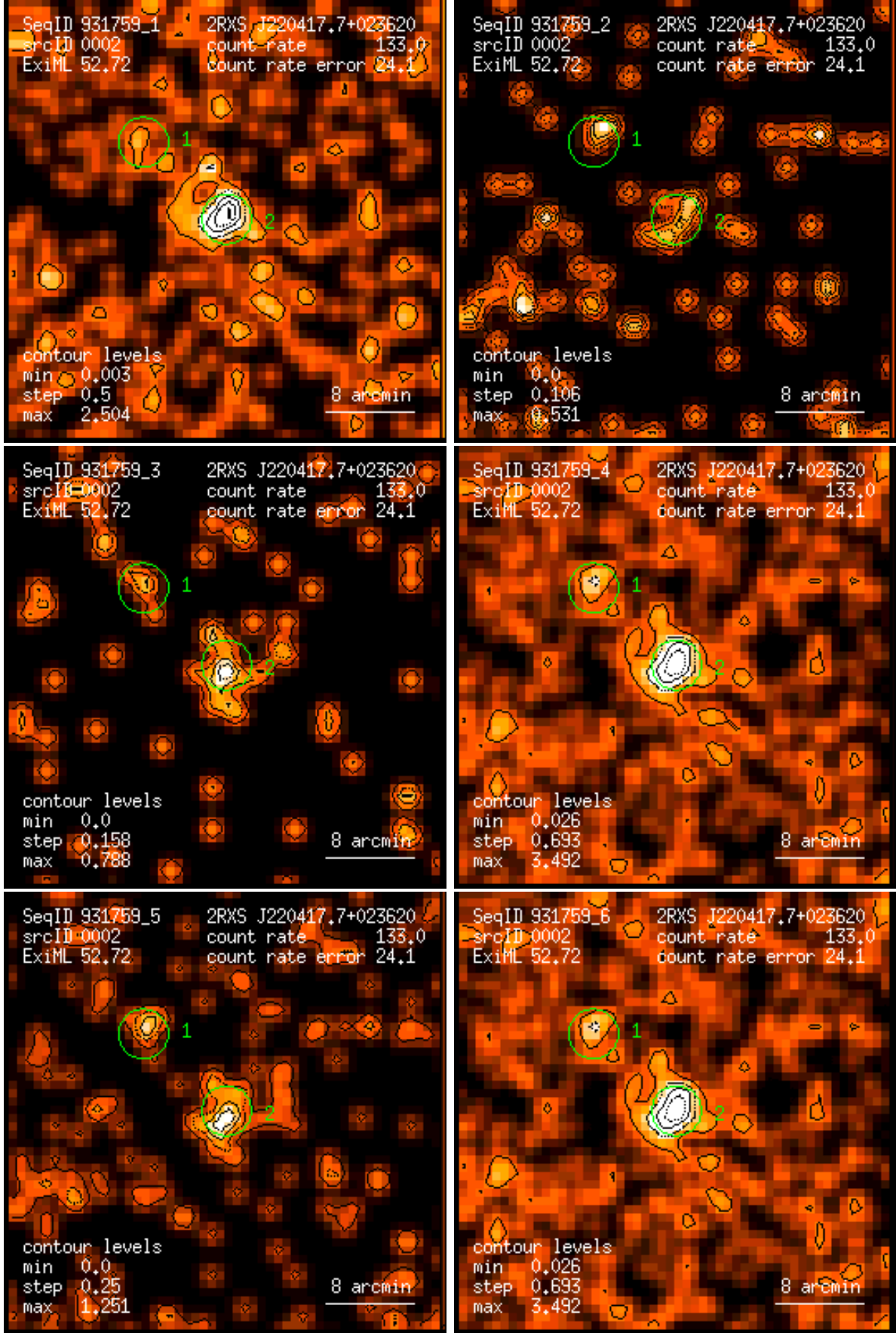
Figure 2: RASS 931759: detection 0002: band rate images, Gaussian filter: (1) PSPC channels 11 – 41, (2) 52 – 90, (3) 91 – 201, (4) 11 – 235, (5) 52 – 201, (6) 11 – 201. Broad band rates in counts/ks. Band rate contour levels in counts/ks/arcmin 2 .
