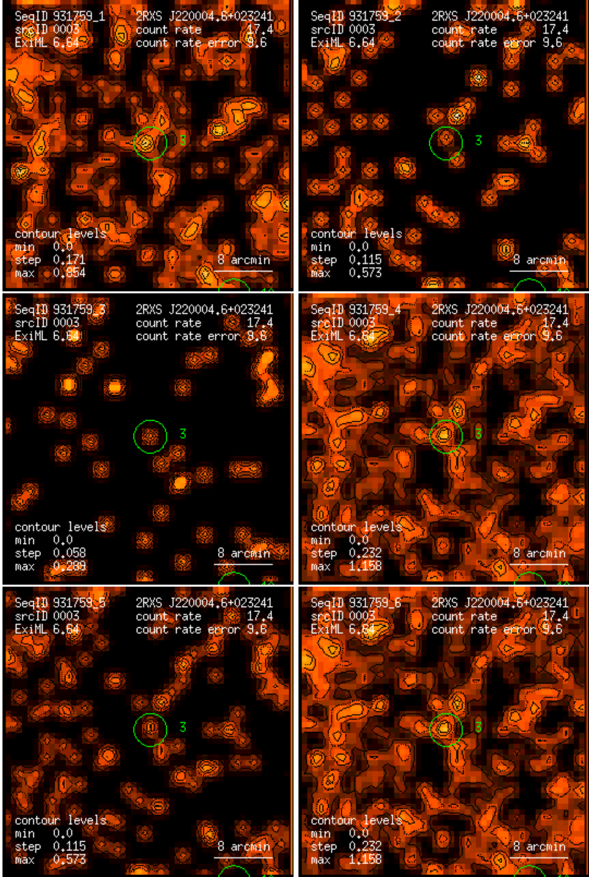
Figure 3: RASS 931759: detection 0003: band rate images, Gaussian filter: (1) PSPC channels 11 – 41, (2) 52 – 90, (3) 91 – 201, (4) 11 – 235, (5) 52 – 201, (6) 11 – 201. Broad band rates in counts/ks. Band rate contour levels in counts/ks/arcmin 2 .
