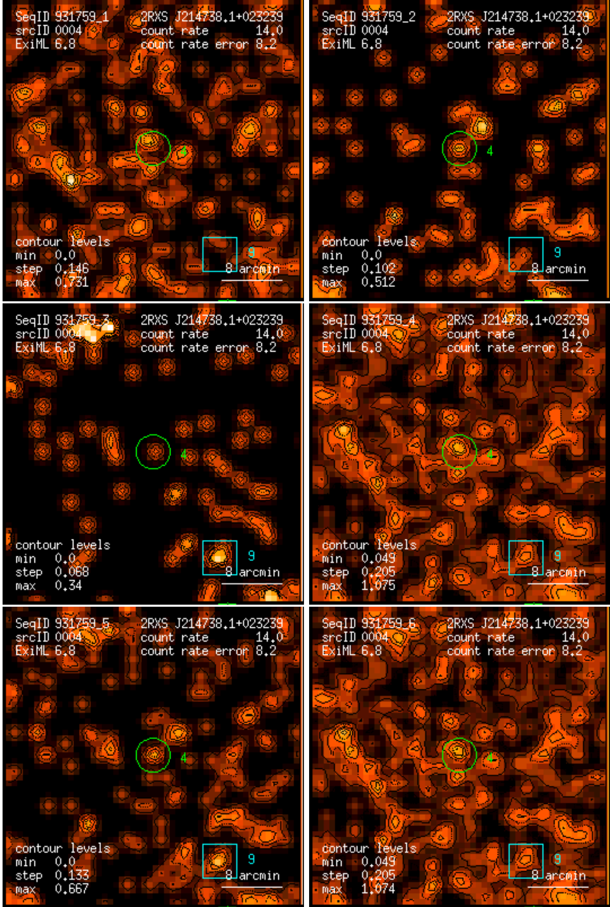
Figure 4: RASS 931759: detection 0004: band rate images, Gaussian filter: (1) PSPC channels 11 – 41, (2) 52 – 90, (3) 91 – 201, (4) 11 – 235, (5) 52 – 201, (6) 11 – 201. Broad band rates in counts/ks. Band rate contour levels in counts/ks/arcmin 2 .
