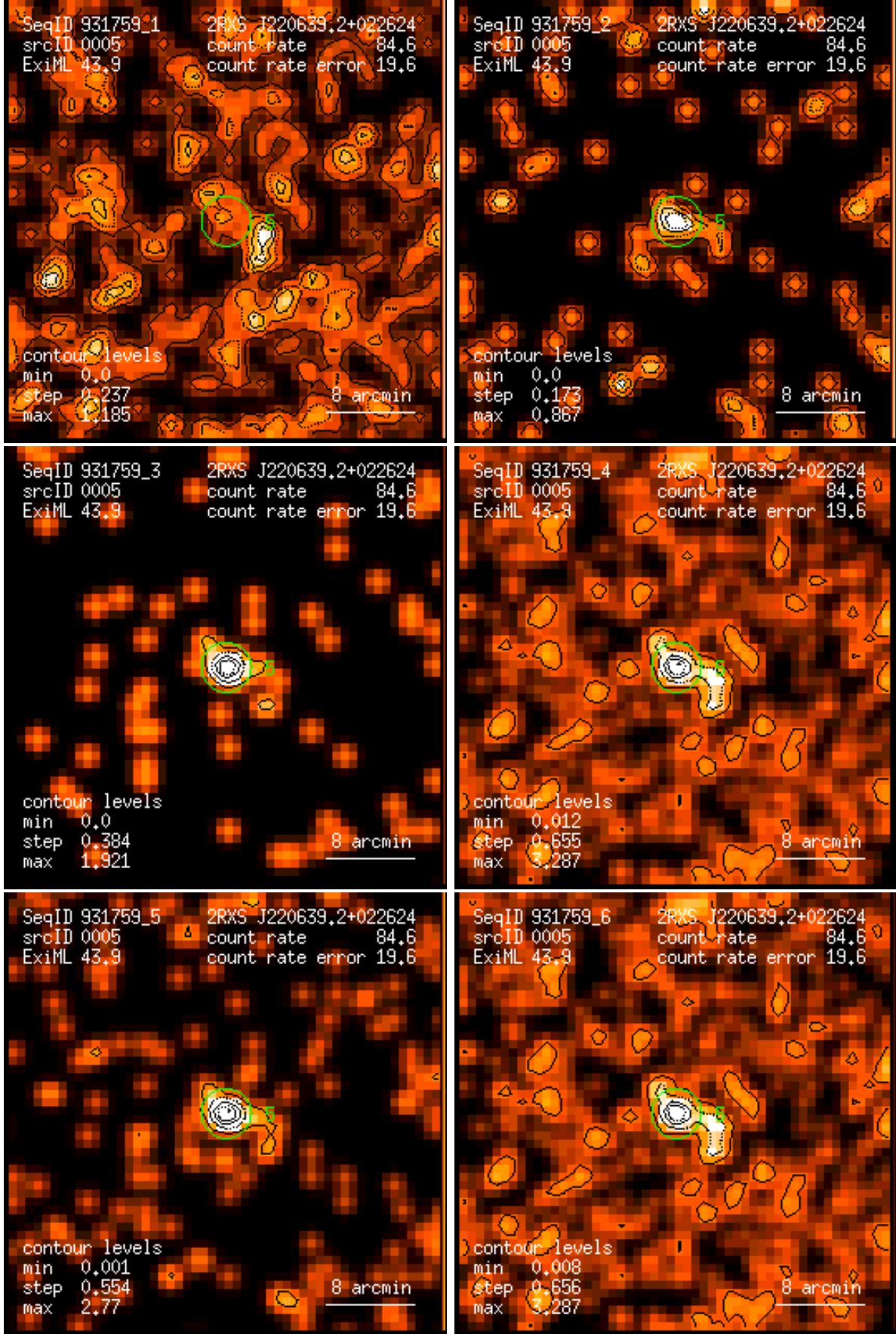
Figure 5: RASS 931759: detection 0005: band rate images, Gaussian filter: (1) PSPC channels 11 – 41, (2) 52 – 90, (3) 91 – 201, (4) 11 – 235, (5) 52 – 201, (6) 11 – 201. Broad band rates in counts/ks. Band rate contour levels in counts/ks/arcmin 2 .
