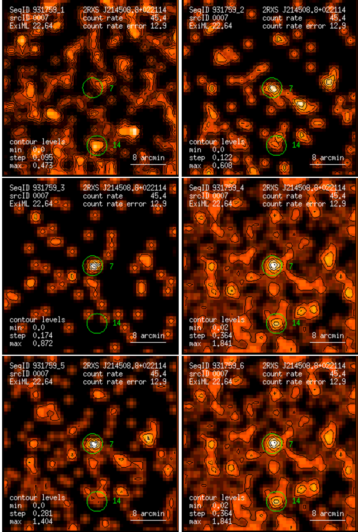
Figure 7: RASS 931759: detection 0007: band rate images, Gaussian filter: (1) PSPC channels 11 – 41, (2) 52 – 90, (3) 91 – 201, (4) 11 – 235, (5) 52 – 201, (6) 11 – 201. Broad band rates in counts/ks. Band rate contour levels in counts/ks/arcmin 2 .
