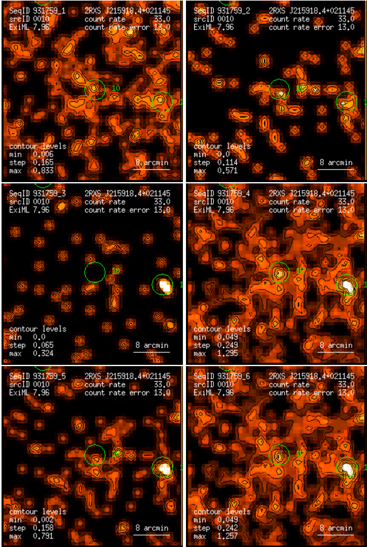
Figure 10: RASS 931759: detection 0010: band rate images, Gaussian filter: (1) PSPC channels 11 – 41, (2) 52 – 90, (3) 91 – 201, (4) 11 – 235, (5) 52 – 201, (6) 11 – 201. Broad band rates in counts/ks. Band rate contour levels in counts/ks/arcmin 2 .
