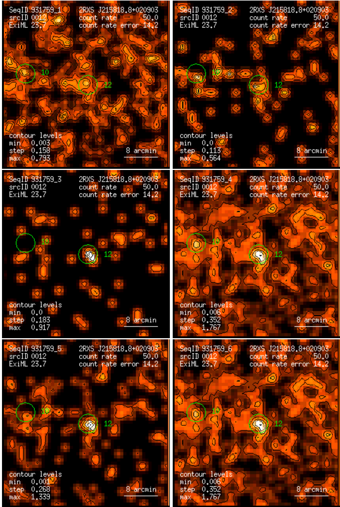
Figure 12: RASS 931759: detection 0012: band rate images, Gaussian filter: (1) PSPC channels 11 – 41, (2) 52 – 90, (3) 91 – 201, (4) 11 – 235, (5) 52 – 201, (6) 11 – 201. Broad band rates in counts/ks. Band rate contour levels in counts/ks/arcmin 2 .
