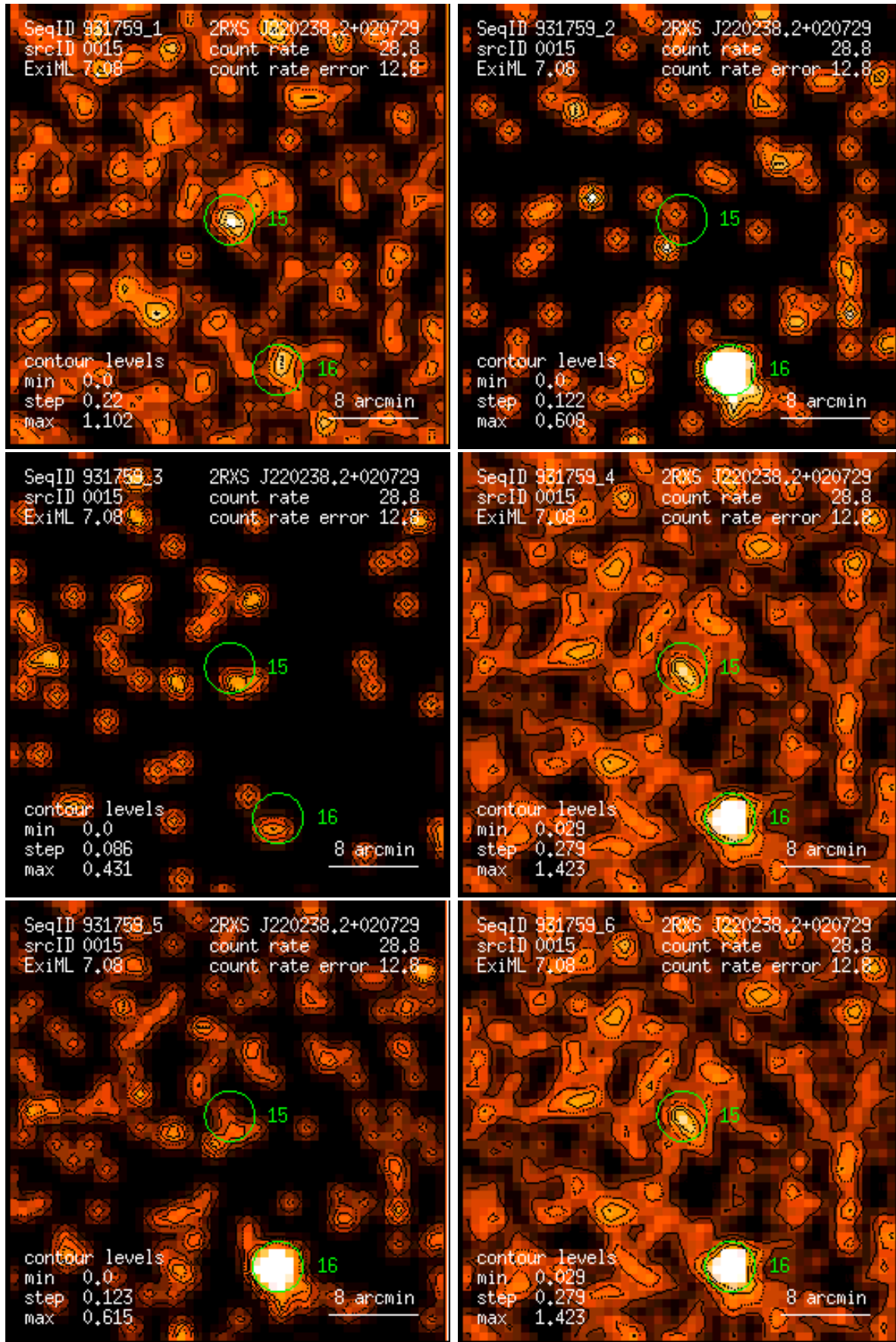
Figure 15: RASS 931759: detection 0015: band rate images, Gaussian filter: (1) PSPC channels 11 – 41, (2) 52 – 90, (3) 91 – 201, (4) 11 – 235, (5) 52 – 201, (6) 11 – 201. Broad band rates in counts/ks. Band rate contour levels in counts/ks/arcmin 2 .
