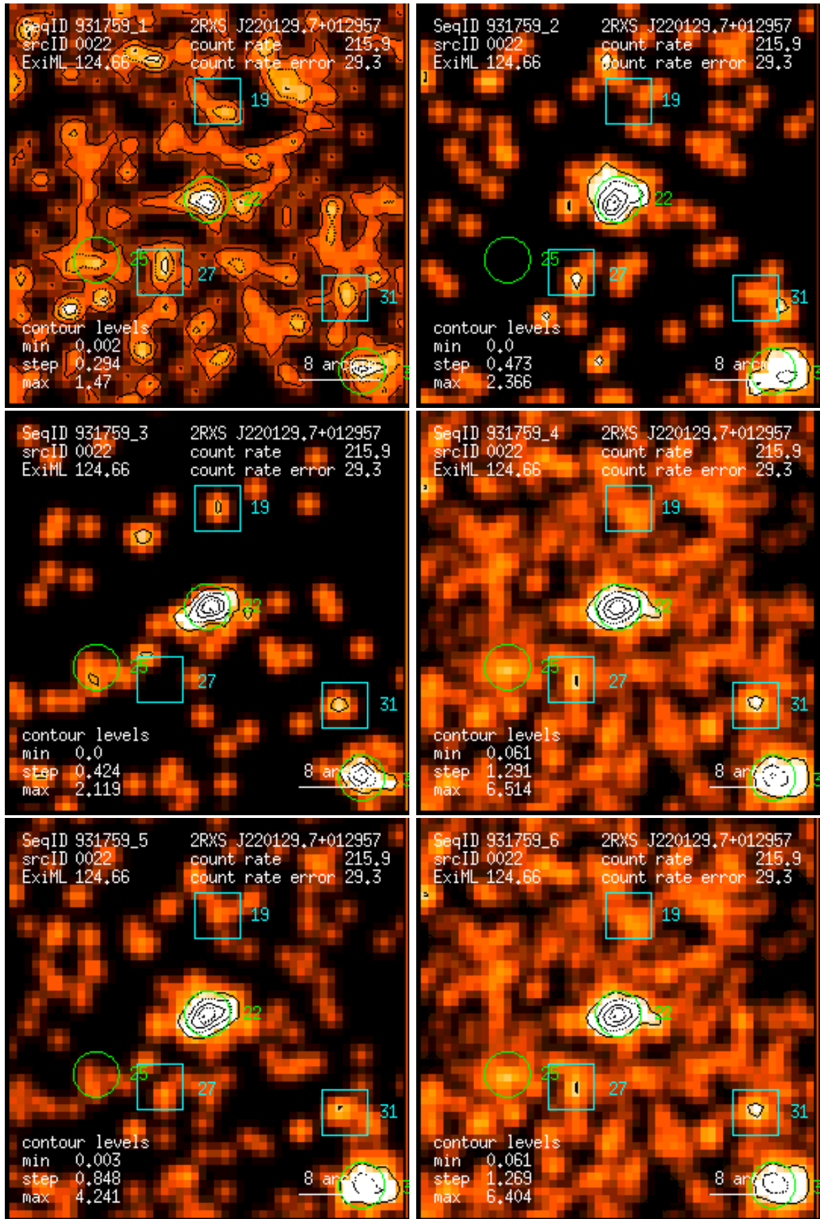
Figure 22: RASS 931759: detection 0022: band rate images, Gaussian filter: (1) PSPC channels 11 – 41, (2) 52 – 90, (3) 91 – 201, (4) 11 – 235, (5) 52 – 201, (6) 11 – 201. Broad band rates in counts/ks. Band rate contour levels in counts/ks/arcmin 2 .
