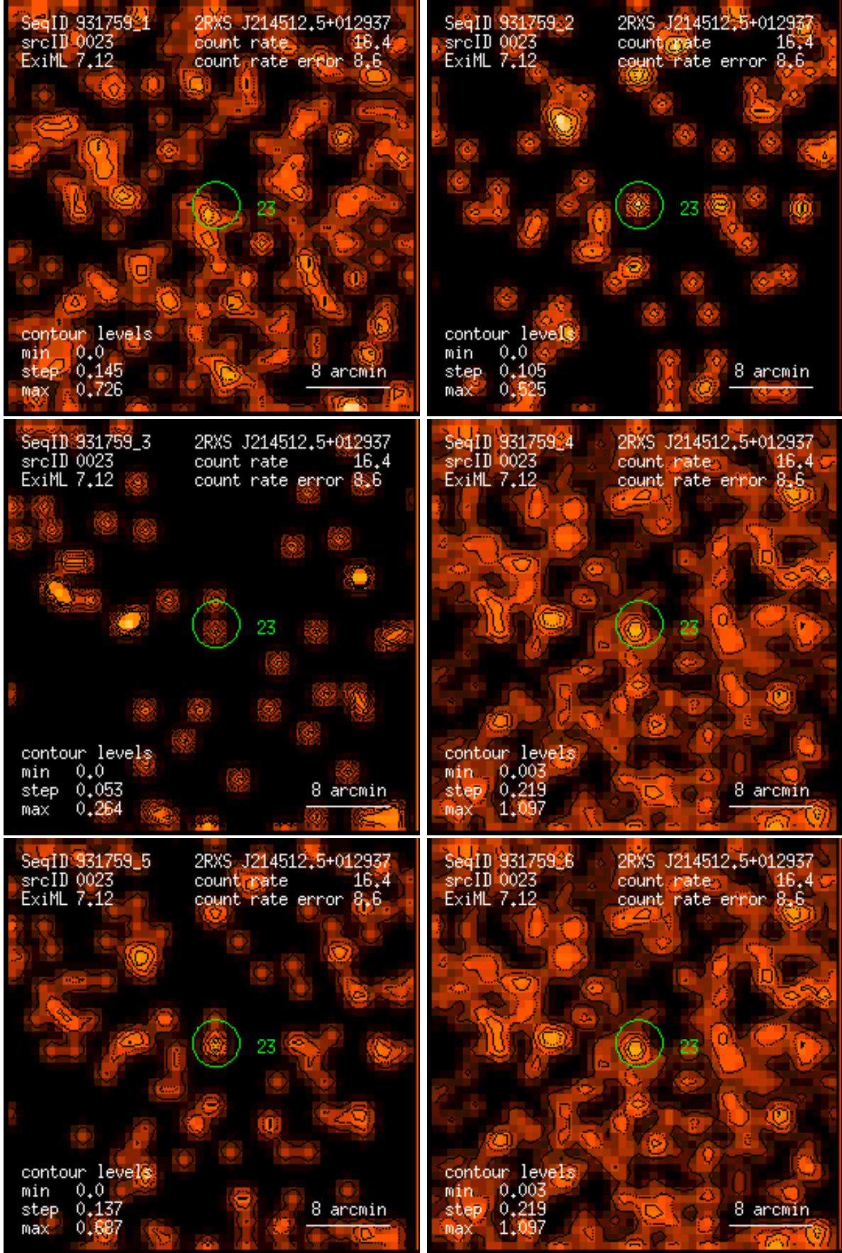
Figure 23: RASS 931759: detection 0023: band rate images, Gaussian filter: (1) PSPC channels 11 – 41, (2) 52 – 90, (3) 91 – 201, (4) 11 – 235, (5) 52 – 201, (6) 11 – 201. Broad band rates in counts/ks. Band rate contour levels in counts/ks/arcmin 2 .
