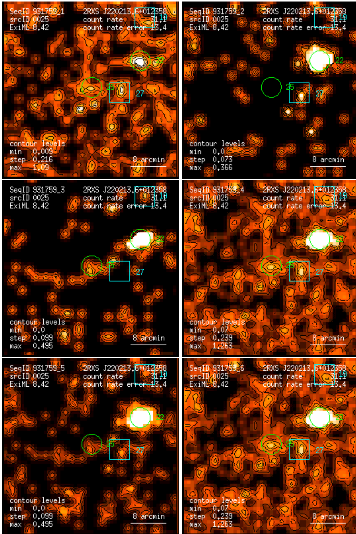
Figure 25: RASS 931759: detection 0025: band rate images, Gaussian filter: (1) PSPC channels 11 – 41, (2) 52 – 90, (3) 91 – 201, (4) 11 – 235, (5) 52 – 201, (6) 11 – 201. Broad band rates in counts/ks. Band rate contour levels in counts/ks/arcmin 2 .
