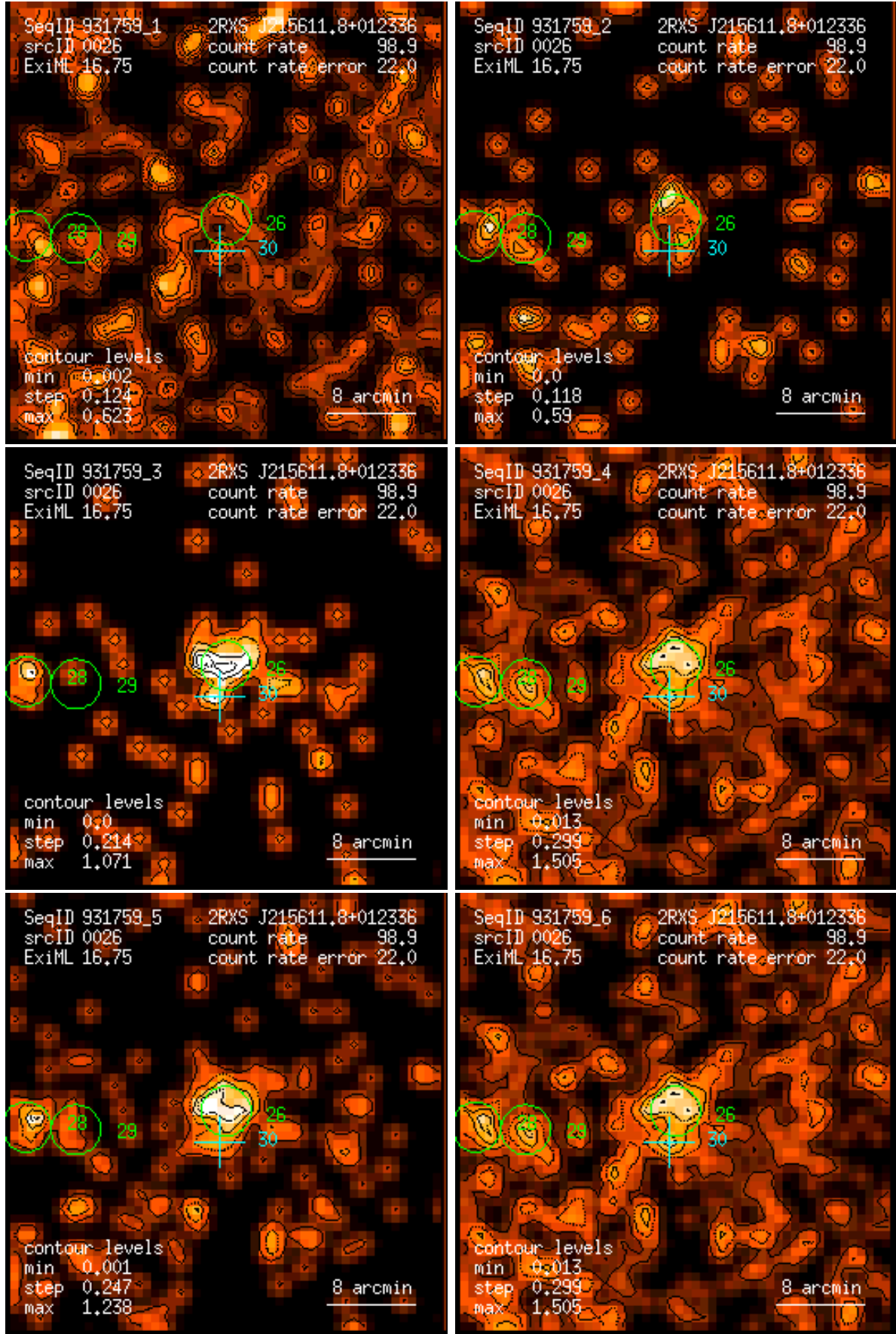
Figure 26: RASS 931759: detection 0026: band rate images, Gaussian filter: (1) PSPC channels 11 – 41, (2) 52 – 90, (3) 91 – 201, (4) 11 – 235, (5) 52 – 201, (6) 11 – 201. Broad band rates in counts/ks. Band rate contour levels in counts/ks/arcmin 2 .
