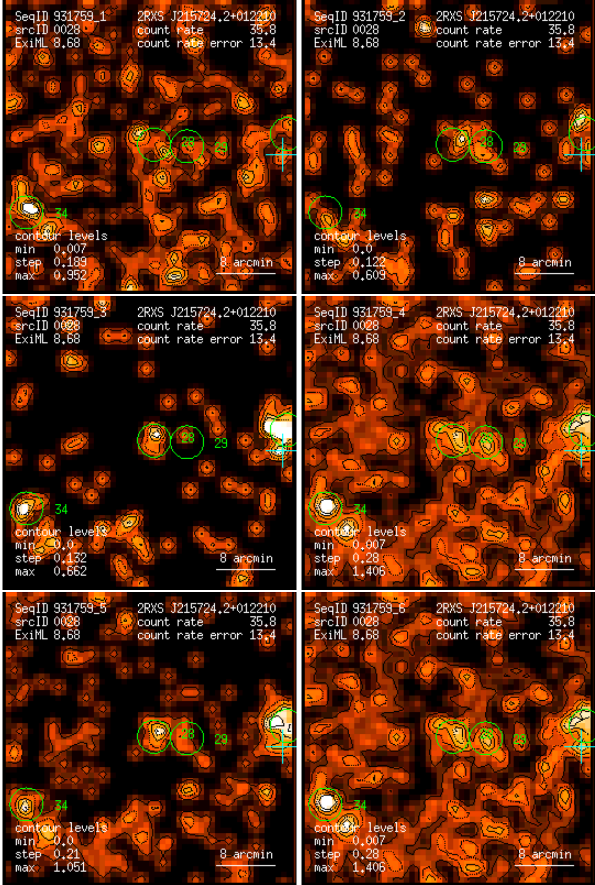
Figure 28: RASS 931759: detection 0028: band rate images, Gaussian filter: (1) PSPC channels 11 – 41, (2) 52 – 90, (3) 91 – 201, (4) 11 – 235, (5) 52 – 201, (6) 11 – 201. Broad band rates in counts/ks. Band rate contour levels in counts/ks/arcmin 2 .
