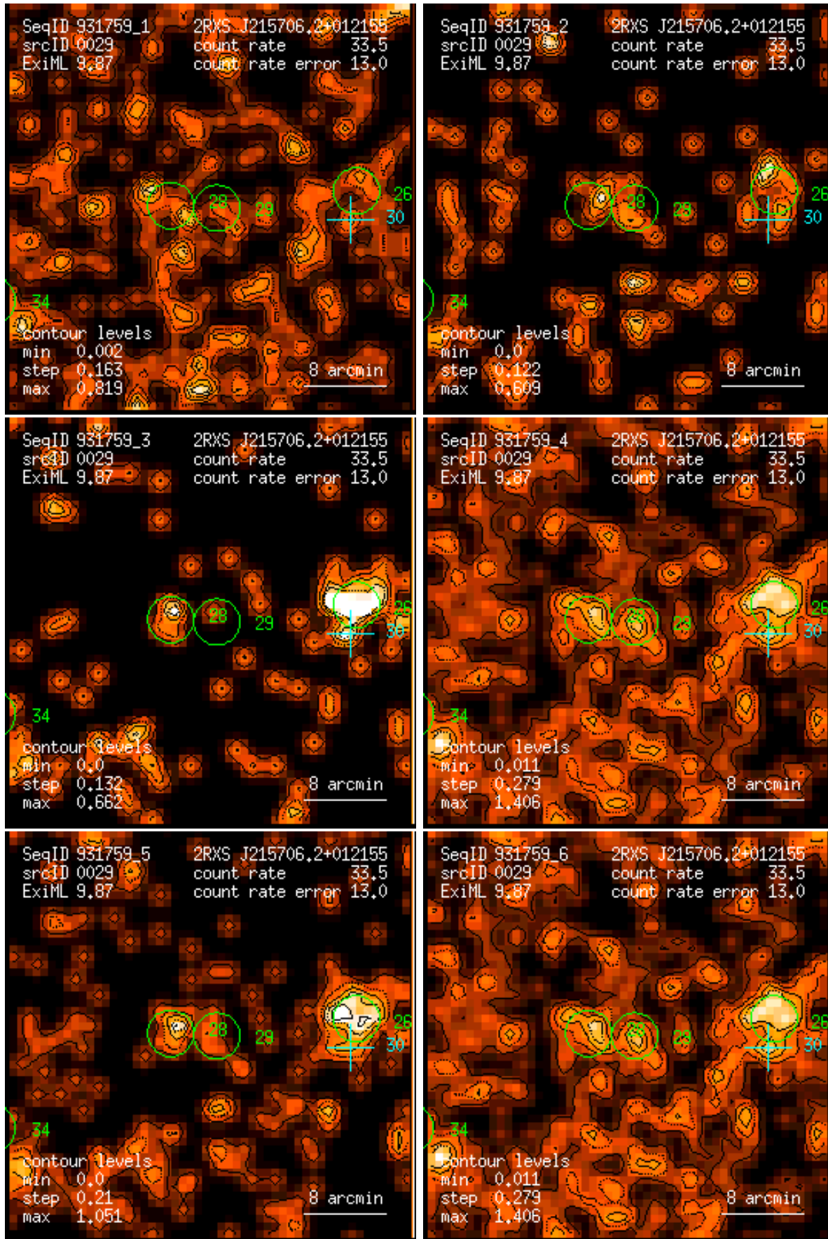
Figure 29: RASS 931759: detection 0029: band rate images, Gaussian filter: (1) PSPC channels 11 – 41, (2) 52 – 90, (3) 91 – 201, (4) 11 – 235, (5) 52 – 201, (6) 11 – 201. Broad band rates in counts/ks. Band rate contour levels in counts/ks/arcmin 2 .
